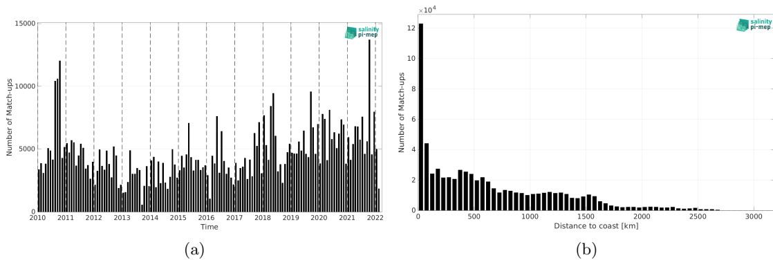
Figure 2: Number of match-ups between TSG (LEGOS-DM) and SMOS SSS L4 v1 - Daily (CMEMS-CNR) SSS as a function of time (a) and as function of the distance to coast (b) over the Equatorial Ocean 10N-10S Pi-MEP region and for the full satellite product period.
