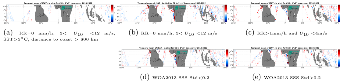
Figure 14: Temporal mean gridded over spatial boxes of size 1^\circ \times 1^\circ of \Delta\text{SSS} (SMOS SSS L4 v1 - Daily (CMEMS-CNR) - TSG (LEGOS-DM)) for 5 different subdatasets corresponding to:RR=0 mm/h, 3 < U_{10} < 12 m/s, SST>5°C, distance to coast > 800 km (a), RR=0 mm/h, 3 < U_{10} < 12 m/s (b), RR>1mm/h and U_{10} < 4 m/s (c), WOA2013 SSS Std<0.2 (d), WOA2013 SSS Std>0.2 (e).
