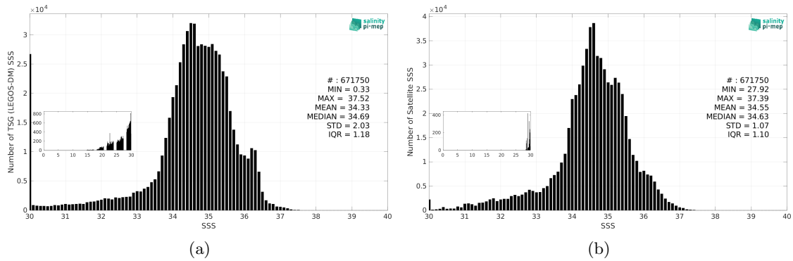
Figure 3: Histograms of SSS from TSG (LEGOS-DM) (a) and SMOS SSS L4 v1 - Daily (CMEMS-CNR) (b) considering all match-up pairs per bins of 0.1 over the Equatorial Ocean 10N-10S Pi-MEP region and for the full satellite product period.
