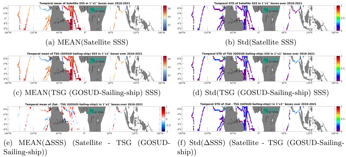
Figure 7: Temporal mean (left) and Std (right) of SSS from SMOS SSS L4 v1 - Daily (CMEMS-CNR) (top), TSG (GOSUD-Sailing-ship) (middle), and of \Delta SSS (Satellite - TSG (GOSUD-Sailing-ship)). Only match-up pairs are used to generate these maps.
