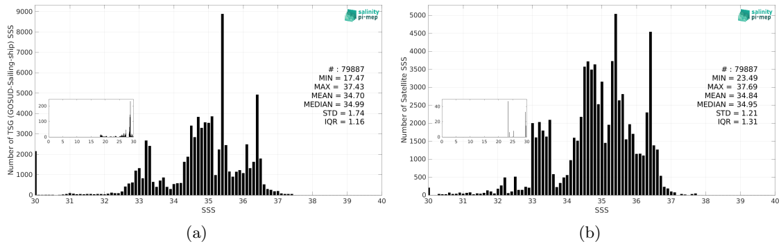
Figure 3: Histograms of SSS from TSG (GOSUD-Sailing-ship) (a) and SMOS SSS L4 v1 - Daily (CMEMS-CNR) (b) considering all match-up pairs per bins of 0.1 over the Equatorial Ocean 10N-10S Pi-MEP region and for the full satellite product period.
