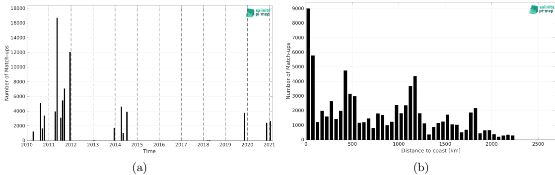
Figure 2: Number of match-ups between TSG (GOSUD-Sailing-ship) and SMOS SSS L4 v1 - Daily (CMEMS-CNR) SSS as a function of time (a) and as function of the distance to coast (b) over the Equatorial Ocean 10N-10S Pi-MEP region and for the full satellite product period.
