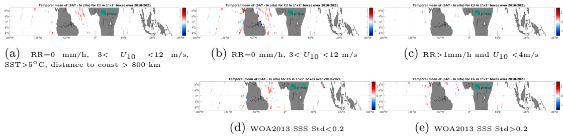
Figure 14: Temporal mean gridded over spatial boxes of size 1^\circ \times 1^\circ of \Delta SSS (SMOS SSS L4 v1 - Daily (CMEMS-CNR) - TSG (GOSUD-Sailing-ship)) for 5 different subdatasets corresponding to: RR=0 mm/h, 3 < U_{10} < 12 m/s, SST>5°C, distance to coast > 800 km (a), RR=0 mm/h, 3 < U_{10} < 12 m/s (b), RR>1mm/h and U_{10} < 4 m/s (c), WOA2013 SSS Std<0.2 (d), WOA2013 SSS Std>0.2 (e).
