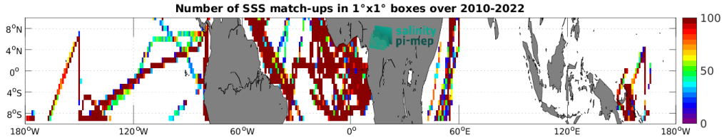
Figure 5: Number of SSS match-ups between TSG (GOSUD-Research-vessel) SSS and the SMOS SSS L4 v1 - Daily (CMEMS-CNR) SSS product for the Equatorial Ocean 10N-10S Pi-MEP region over 1^\circ \times 1^\circ boxes and for the full satellite product period.
