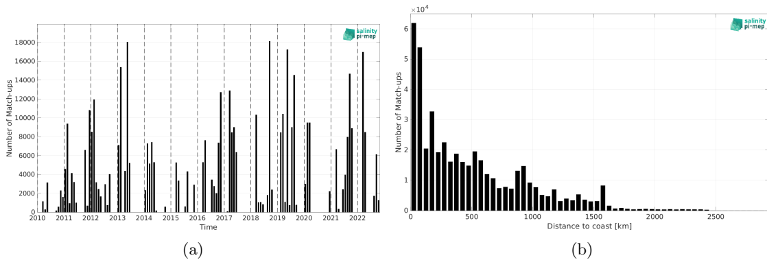
Figure 2: Number of match-ups between TSG (GOSUD-Research-vessel) and SMOS SSS L4 v1 - Daily (CMEMS-CNR) SSS as a function of time (a) and as function of the distance to coast (b) over the Equatorial Ocean 10N-10S Pi-MEP region and for the full satellite product period.
