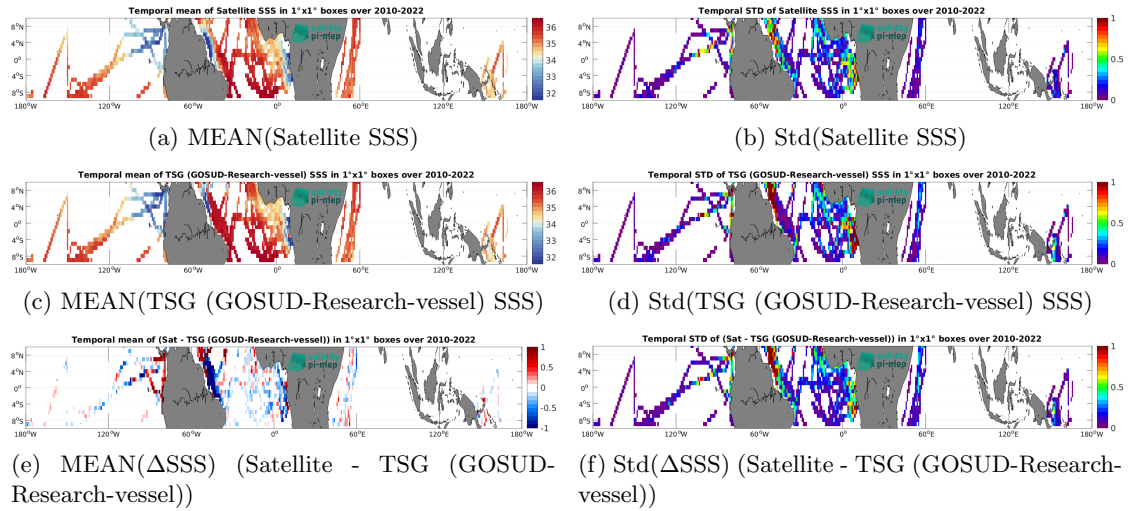
Figure 7: Temporal mean (left) and Std (right) of SSS from SMOS SSS L4 v1 - Daily (CMEMS-CNR) (top), TSG (GOSUD-Research-vessel) (middle), and of \Delta SSS (Satellite - TSG (GOSUD-Research-vessel)). Only match-up pairs are used to generate these maps.
