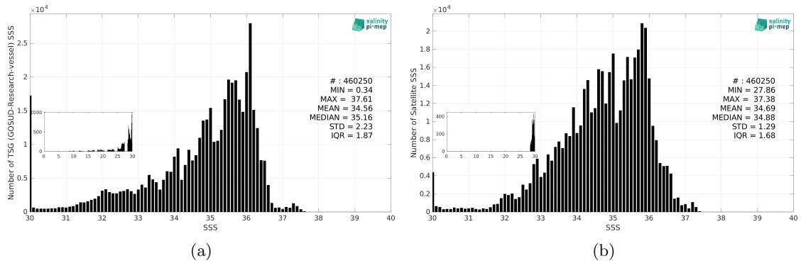
Figure 3: Histograms of SSS from TSG (GOSUD-Research-vessel) (a) and SMOS SSS L4 v1 - Daily (CMEMS-CNR) (b) considering all match-up pairs per bins of 0.1 over the Equatorial Ocean 10N-10S Pi-MEP region and for the full satellite product period.
