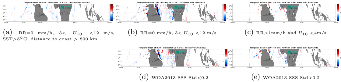
Figure 14: Temporal mean gridded over spatial boxes of size 1^\circ \times 1^\circ of \Delta SSS (SMOS SSS L4 v1 - Daily (CMEMS-CNR) - TSG (GOSUD-Research-vessel)) for 5 different subdatasets corresponding to: RR=0 mm/h, 3 < U_{10} < 12 m/s, SST>5°C, distance to coast > 800 km (a), RR=0 mm/h, 3 < U_{10} < 12 m/s (b), RR>1mm/h and U_{10} < 4 m/s (c), WOA2013 SSS Std<0.2 (d), WOA2013 SSS Std>0.2 (e).
