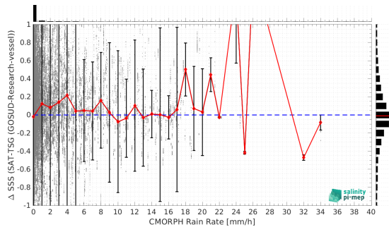
(e) CMORPH Rain rate
