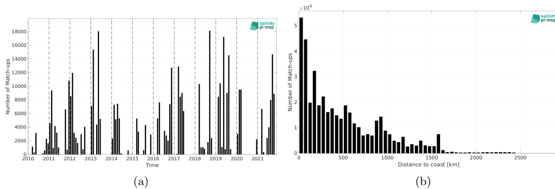
Figure 2: Number of match-ups between TSG (GOSUD-Research-vessel) and SMOS SSS L4 v1 - Daily (CMEMS-CNR) SSS as a function of time (a) and as function of the distance to coast (b) over the Equatorial Ocean 10N-10S Pi-MEP region and for the full satellite product period.
