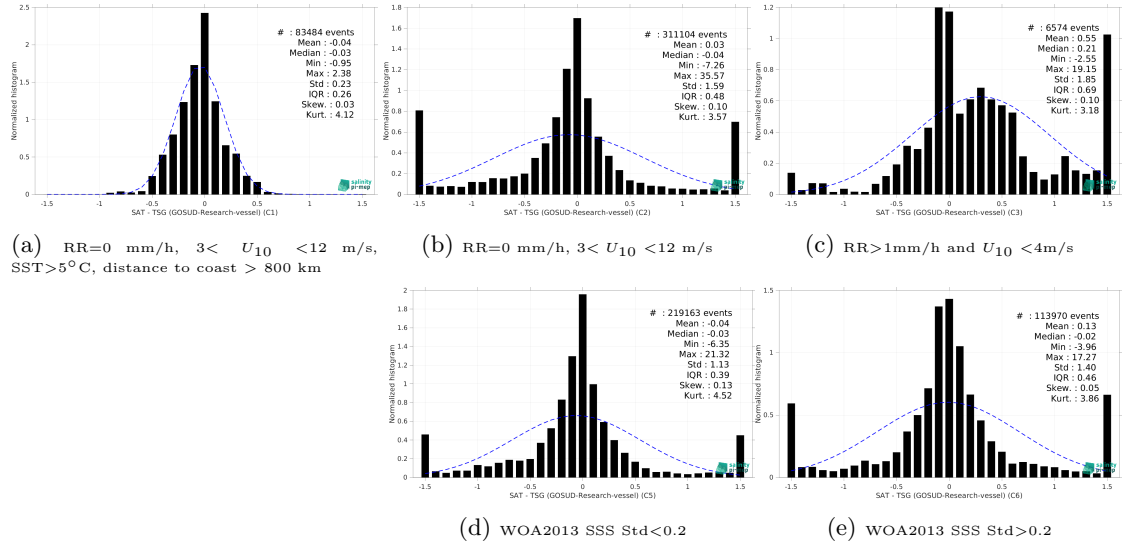
Figure 15: Normalized histogram of \Delta\text{SSS} (SMOS SSS L4 v1 - Daily (CMEMS-CNR) - TSG (GOSUD-Research-vessel)) for 5 different subdatasets corresponding to: RR=0 mm/h, 3 < U_{10} < 12 m/s, SST>5°C, distance to coast > 800 km (a), RR=0 mm/h, 3 < U_{10} < 12 m/s (b), RR>1mm/h and U_{10} < 4 m/s (c), WOA2013 SSS Std<0.2 (d), WOA2013 SSS Std>0.2 (e).
