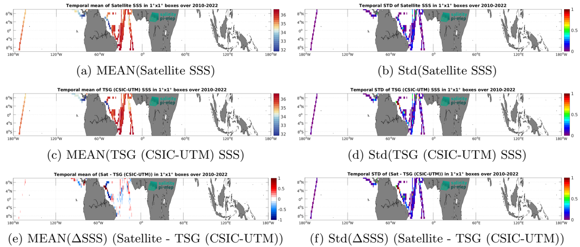
Figure 7: Temporal mean (left) and Std (right) of SSS from SMOS SSS L4 v1 - Daily (CMEMS-CNR) (top), TSG (CSIC-UTM) (middle), and of \Delta SSS (Satellite - TSG (CSIC-UTM)). Only match-up pairs are used to generate these maps.
