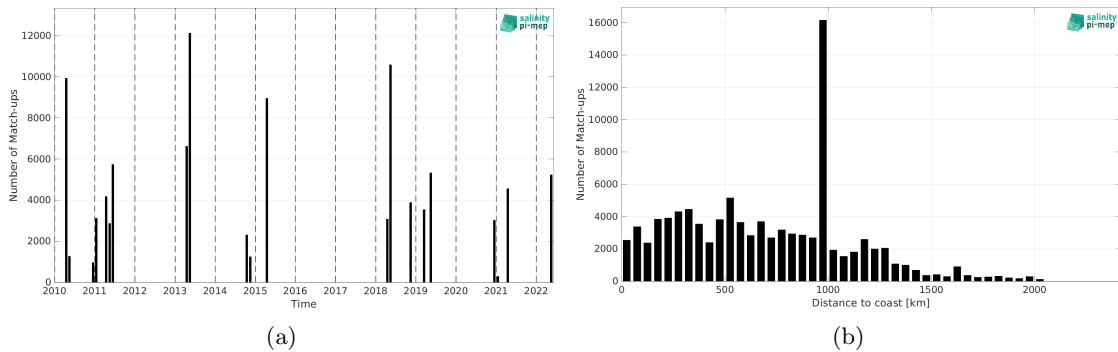
Figure 2: Number of match-ups between TSG (CSIC-UTM) and SMOS SSS L4 v1 - Daily (CMEMS-CNR) SSS as a function of time (a) and as function of the distance to coast (b) over the Equatorial Ocean 10N-10S Pi-MEP region and for the full satellite product period.
