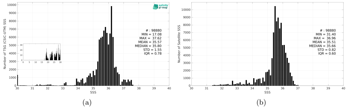
Figure 3: Histograms of SSS from TSG (CSIC-UTM) (a) and SMOS SSS L4 v1 - Daily (CMEMS-CNR) (b) considering all match-up pairs per bins of 0.1 over the Equatorial Ocean 10N-10S Pi-MEP region and for the full satellite product period.
