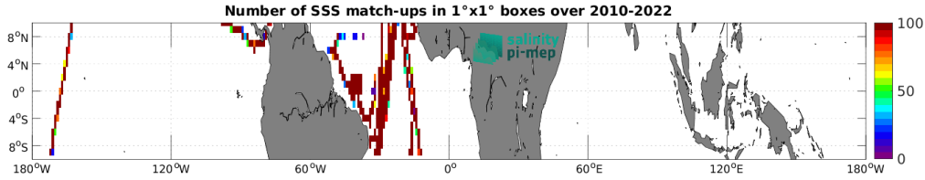
Figure 5: Number of SSS match-ups between TSG (CSIC-UTM) SSS and the SMOS SSS L4 v1 - Daily (CMEMS-CNR) SSS product for the Equatorial Ocean 10N-10S Pi-MEP region over 1^\circ \times 1^\circ boxes and for the full satellite product period.
