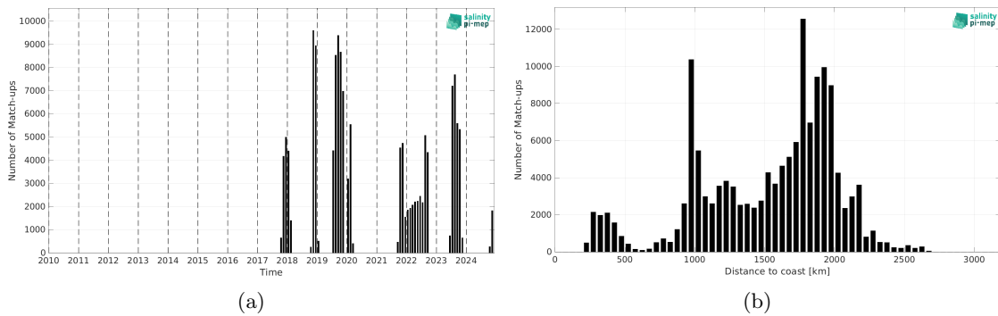
Figure 2: Number of match-ups between Saildrone and SMOS SSS L4 v1 - Daily (CMEMS-CNR) SSS as a function of time (a) and as function of the distance to coast (b) over the Equatorial Ocean 10N-10S Pi-MEP region and for the full satellite product period.
