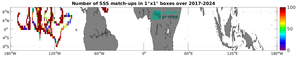
Figure 5: Number of SSS match-ups between Saildrone SSS and the SMOS SSS L4 v1 - Daily (CMEMS-CNR) SSS product for the Equatorial Ocean 10N-10S Pi-MEP region over 1^\circ \times 1^\circ boxes and for the full satellite product period.
