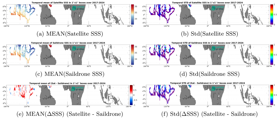
Figure 7: Temporal mean (left) and Std (right) of SSS from SMOS SSS L4 v1 - Daily (CMEMS-CNR) (top), Saildrone (middle), and of \Delta SSS (Satellite - Saildrone). Only match-up pairs are used to generate these maps.
