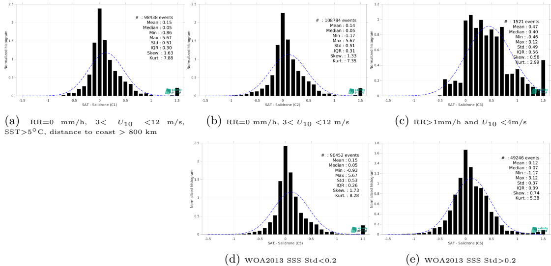
Figure 15: Normalized histogram of \Delta SSS (SMOS SSS L4 v1 - Daily (CMEMS-CNR) - Saildrone) for 5 different subdatasets corresponding to: RR=0 mm/h, 3 < U_{10} < 12 m/s, SST>5°C, distance to coast > 800 km (a), RR=0 mm/h, 3 < U_{10} < 12 m/s (b), RR>1mm/h and U_{10} < 4 m/s (c), WOA2013 SSS Std<0.2 (d), WOA2013 SSS Std>0.2 (e).
