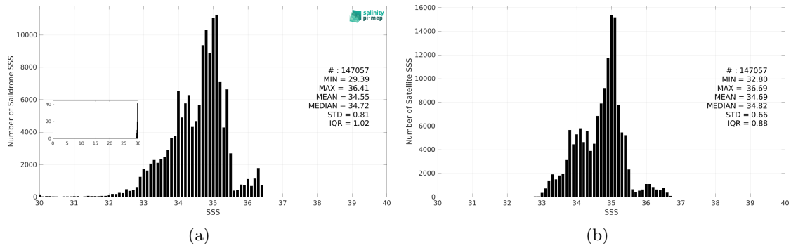
Figure 3: Histograms of SSS from Saildrone (a) and SMOS SSS L4 v1 - Daily (CMEMS-CNR) (b) considering all match-up pairs per bins of 0.1 over the Equatorial Ocean 10N-10S Pi-MEP region and for the full satellite product period.
