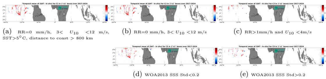
Figure 14: Temporal mean gridded over spatial boxes of size 1^\circ \times 1^\circ of \Delta SSS (SMOS SSS L4 v1 - Daily (CMEMS-CNR) - Saildrone) for 5 different subdatasets corresponding to: RR=0 mm/h, 3 < U_{10} < 12 m/s, SST>5°C, distance to coast > 800 km (a), RR=0 mm/h, 3 < U_{10} < 12 m/s (b), RR>1mm/h and U_{10} < 4 m/s (c), WOA2013 SSS Std<0.2 (d), WOA2013 SSS Std>0.2 (e).
