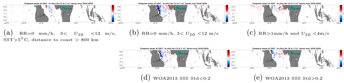
Figure 13: Temporal mean gridded over spatial boxes of size 1^\circ \times 1^\circ of \Delta SSS (SMOS SSS L4 v1 - Daily (CMEMS-CNR) - Surface drifters) for 5 different subdatasets corresponding to: RR=0 mm/h, 3 < U_{10} < 12 m/s, SST >5^\circ C, distance to coast > 800 km (a), RR=0 mm/h, 3 < U_{10} < 12 m/s (b), RR >1 mm/h and U_{10} < 4 m/s (c), WOA2013 SSS Std <0.2 (d), WOA2013 SSS Std >0.2 (e).
