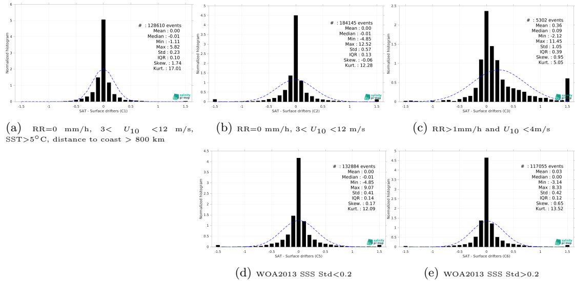
Figure 14: Normalized histogram of \Delta SSS (SMOS SSS L4 v1 - Daily (CMEMS-CNR) - Surface drifters) for 5 different subdatasets corresponding to: RR=0 mm/h, 3 < U_{10} < 12 m/s, SST >5^\circ C, distance to coast > 800 km (a), RR=0 mm/h, 3 < U_{10} < 12 m/s (b), RR >1 mm/h and U_{10} < 4 m/s (c), WOA2013 SSS Std <0.2 (d), WOA2013 SSS Std >0.2 (e).
