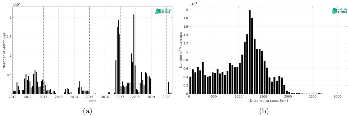
Figure 2: Number of match-ups between Surface drifters and SMOS SSS L4 v1 - Daily (CMEMS-CNR) SSS as a function of time (a) and as function of the distance to coast (b) over the Equatorial Ocean 10N-10S Pi-MEP region and for the full satellite product period.
