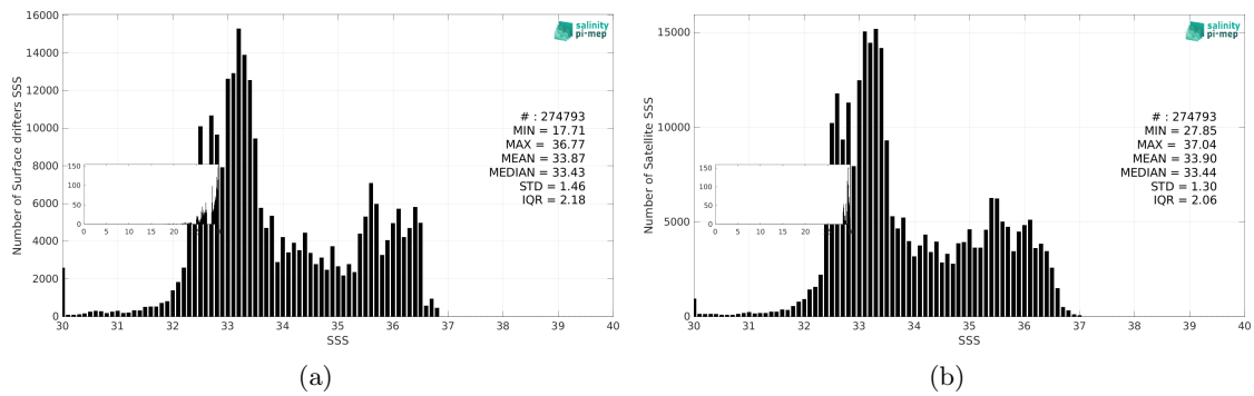
Figure 3: Histograms of SSS from Surface drifters (a) and SMOS SSS L4 v1 - Daily (CMEMS-CNR) (b) considering all match-up pairs per bins of 0.1 over the Equatorial Ocean 10N-10S Pi-MEP region and for the full satellite product period.
