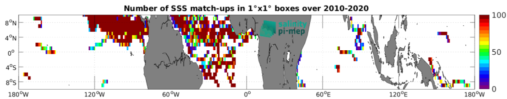
Figure 4: Number of SSS match-ups between Surface drifters SSS and the SMOS SSS L4 v1 - Daily (CMEMS-CNR) SSS product for the Equatorial Ocean 10N-10S Pi-MEP region over 1^\circ \times 1^\circ boxes and for the full satellite product period.
