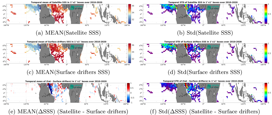
Figure 6: Temporal mean (left) and Std (right) of SSS from SMOS SSS L4 v1 - Daily (CMEMS-CNR) (top), Surface drifters (middle), and of \Delta SSS (Satellite - Surface drifters). Only match-up pairs are used to generate these maps.
