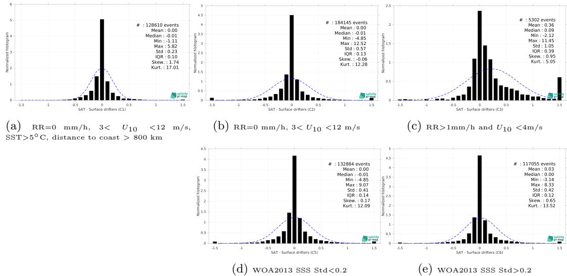
Figure 14: Normalized histogram of \Delta SSS (SMOS SSS L4 v1 - Daily (CMEMS-CNR) - Surface drifters) for 5 different subdatasets corresponding to: RR=0 mm/h, 3 < U_{10} < 12 m/s, SST > 5^\circ\text{C} , distance to coast > 800 km (a), RR=0 mm/h, 3 < U_{10} < 12 m/s (b), RR > 1 mm/h and U_{10} < 4 m/s (c), WOA2013 SSS Std < 0.2 (d), WOA2013 SSS Std > 0.2 (e).
