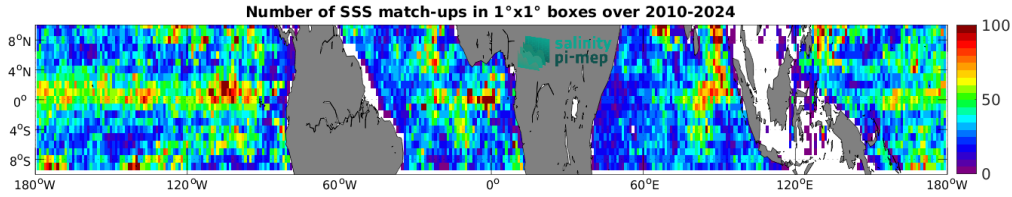
Figure 5: Number of SSS match-ups between Argo SSS and the SMOS SSS L4 v1 - Daily (CMEMS-CNR) SSS product for the Equatorial Ocean 10N-10S Pi-MEP region over 1^\circ \times 1^\circ boxes and for the full satellite product period.
