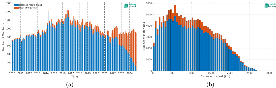
Figure 2: Number of match-ups between Argo and SMOS SSS L4 v1 - Daily (CMEMS-CNR) SSS as a function of time (a) and as function of the distance to coast (b) over the Equatorial Ocean 10N-10S Pi-MEP region and for the full satellite product period.
