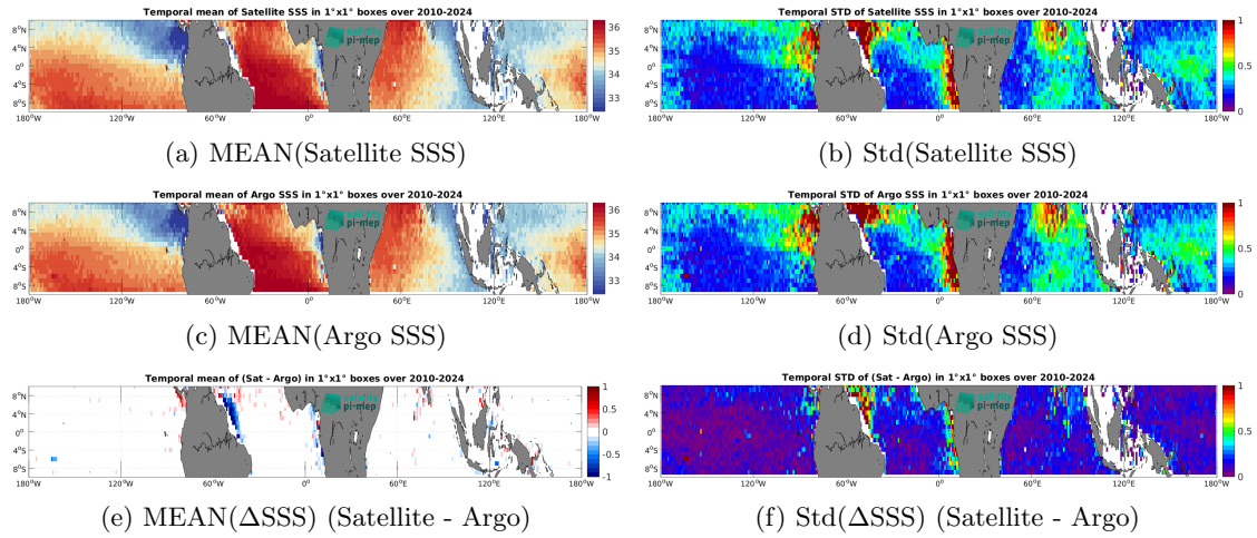
Figure 7: Temporal mean (left) and Std (right) of SSS from SMOS SSS L4 v1 - Daily (CMEMS-CNR) (top), Argo (middle), and of \Delta SSS (Satellite - Argo). Only match-up pairs are used to generate these maps.
