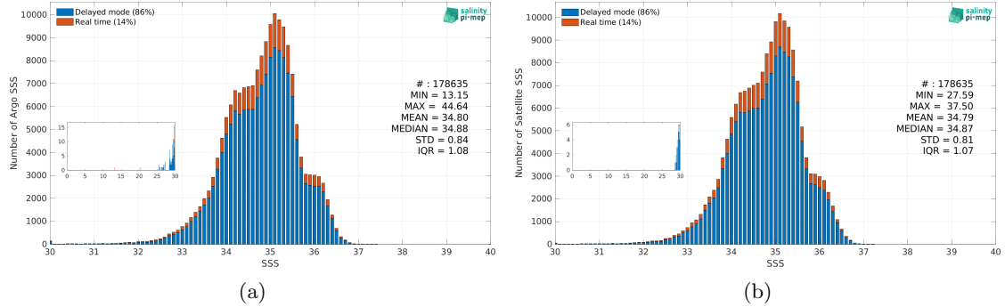
Figure 3: Histograms of SSS from Argo (a) and SMOS SSS L4 v1 - Daily (CMEMS-CNR) (b) considering all match-up pairs per bins of 0.1 over the Equatorial Ocean 10N-10S Pi-MEP region and for the full satellite product period.
