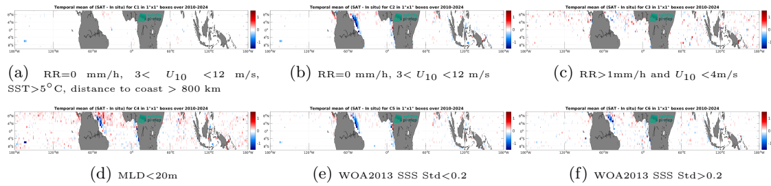
Figure 14: Temporal mean gridded over spatial boxes of size 1^\circ \times 1^\circ of \Delta SSS (SMOS SSS L4 v1 - Daily (CMEMS-CNR) - Argo) for 6 different subdatasets corresponding to:RR=0 mm/h, 3 < U_{10} < 12 m/s, SST >5^\circ\text{C} , distance to coast > 800 km (a), RR=0 mm/h, 3 < U_{10} < 12 m/s (b), RR >1 mm/h and U_{10} < 4 m/s (c),MLD <20 m (d),WOA2013 SSS Std <0.2 (e),WOA2013 SSS Std >0.2 (f).
