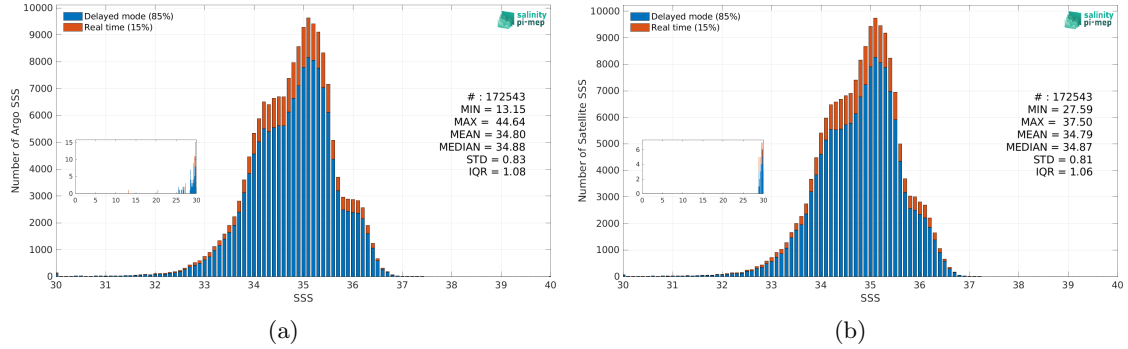
Figure 3: Histograms of SSS from Argo (a) and SMOS SSS L4 v1 - Daily (CMEMS-CNR) (b) considering all match-up pairs per bins of 0.1 over the Equatorial Ocean 10N-10S Pi-MEP region and for the full satellite product period.
