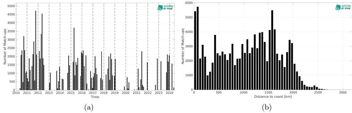
Figure 2: Number of match-ups between TSG (SAMOS) and SMOS SSS L4 OI v346 - Weekly (CMEMS-CATDS-LOPS) SSS as a function of time (a) and as function of the distance to coast (b) over the Equatorial Ocean 10N-10S Pi-MEP region and for the full satellite product period.
