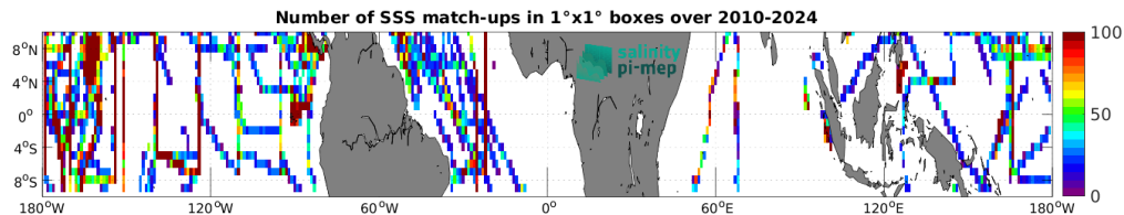
Figure 5: Number of SSS match-ups between TSG (SAMOS) SSS and the SMOS SSS L4 OI v346 - Weekly (CMEMS-CATDS-LOPS) SSS product for the Equatorial Ocean 10N-10S Pi-MEP region over 1^\circ \times 1^\circ boxes and for the full satellite product period.
