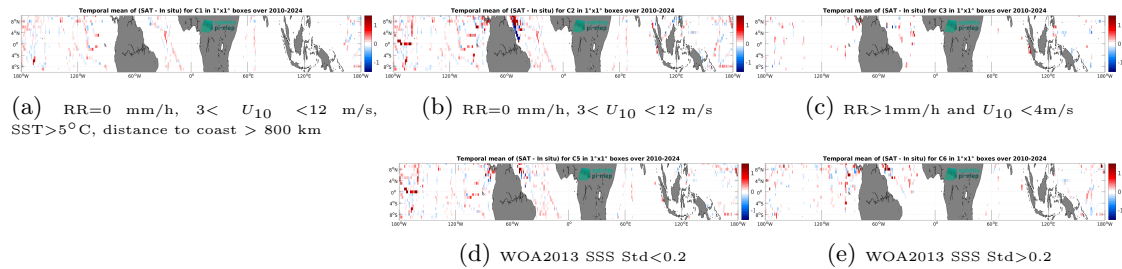
Figure 14: Temporal mean gridded over spatial boxes of size 1^\circ \times 1^\circ of \Delta SSS (SMOS SSS L4 OI v346 - Weekly (CMEMS-CATDS-LOPS) - TSG (SAMOS)) for 5 different subdatasets corresponding to: RR=0 mm/h, 3 < U_{10} < 12 m/s, SST>5°C, distance to coast > 800 km (a), RR=0 mm/h, 3 < U_{10} < 12 m/s (b), RR>1mm/h and U_{10} < 4 m/s (c), WOA2013 SSS Std<0.2 (d), WOA2013 SSS Std>0.2 (e).
