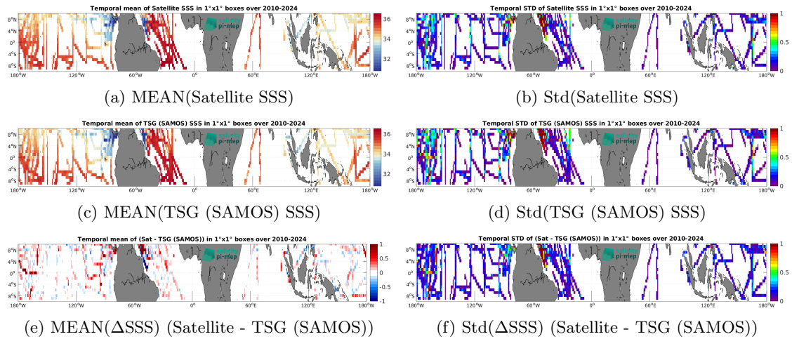
Figure 7: Temporal mean (left) and Std (right) of SSS from SMOS SSS L4 OI v346 - Weekly (CMEMS-CATDS-LOPS) (top), TSG (SAMOS) (middle), and of \Delta SSS (Satellite - TSG (SAMOS)). Only match-up pairs are used to generate these maps.
