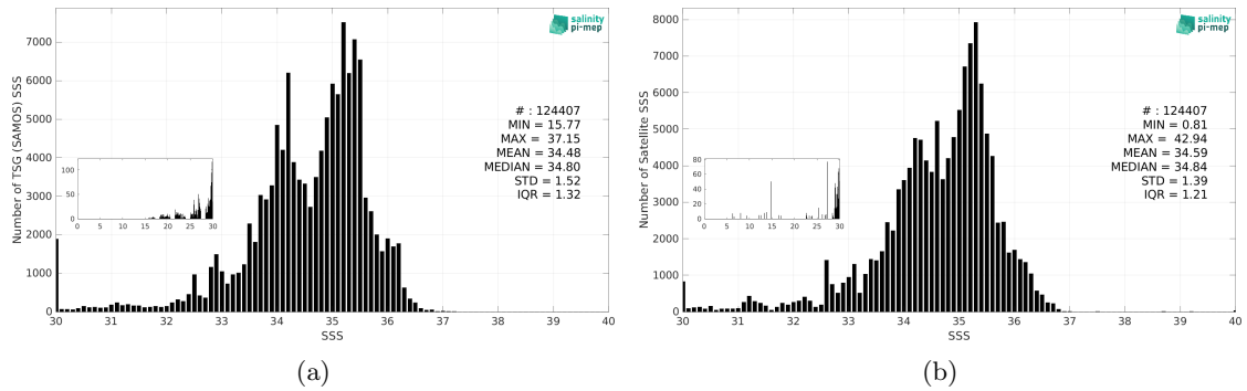
Figure 3: Histograms of SSS from TSG (SAMOS) (a) and SMOS SSS L4 OI v346 - Weekly (CMEMS-CATDS-LOPS) (b) considering all match-up pairs per bins of 0.1 over the Equatorial Ocean 10N-10S Pi-MEP region and for the full satellite product period.
