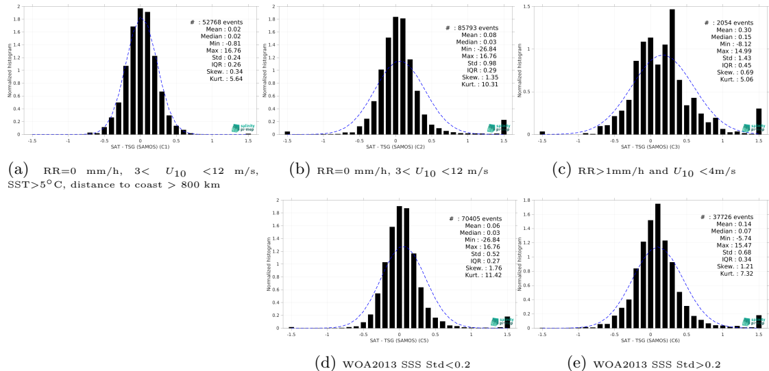
Figure 15: Normalized histogram of \Delta\text{SSS} (SMOS SSS L4 OI v346 - Weekly (CMEMS-CATDS-LOPS) - TSG (SAMOS)) for 5 different subdatasets corresponding to: RR=0 mm/h, 3 < U_{10} < 12 m/s, SST>5°C, distance to coast > 800 km (a), RR=0 mm/h, 3 < U_{10} < 12 m/s (b), RR>1mm/h and U_{10} < 4 m/s (c), WOA2013 SSS Std<0.2 (d), WOA2013 SSS Std>0.2 (e).
