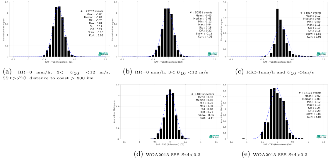
Figure 15: Normalized histogram of \Delta SSS (SMOS SSS L4 OI v346 - Weekly (CMEMS-CATDS-LOPS) - TSG (Polarstern)) for 5 different subdatasets corresponding to: RR=0 mm/h, 3 < U_{10} < 12 m/s, SST>5°C, distance to coast > 800 km (a), RR=0 mm/h, 3 < U_{10} < 12 m/s (b), RR>1mm/h and U_{10} < 4 m/s (c), WOA2013 SSS Std<0.2 (d), WOA2013 SSS Std>0.2 (e).
