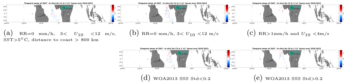
Figure 14: Temporal mean gridded over spatial boxes of size 1^\circ \times 1^\circ of \Delta SSS (SMOS SSS L4 OI v346 - Weekly (CMEMS-CATDS-LOPS) - TSG (Polarstern)) for 5 different subdatasets corresponding to:RR=0 mm/h, 3 < U_{10} < 12 m/s, SST>5°C, distance to coast > 800 km (a), RR=0 mm/h, 3 < U_{10} < 12 m/s (b), RR>1mm/h and U_{10} < 4 m/s (c), WOA2013 SSS Std<0.2 (d), WOA2013 SSS Std>0.2 (e).
