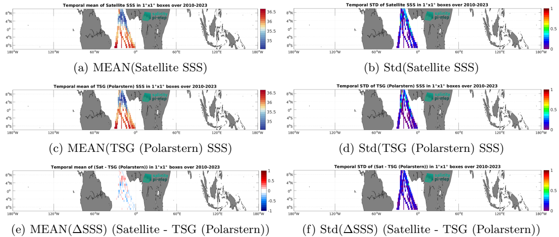
Figure 7: Temporal mean (left) and Std (right) of SSS from SMOS SSS L4 OI v346 - Weekly (CMEMS-CATDS-LOPS) (top), TSG (Polarstern) (middle), and of \Delta SSS (Satellite - TSG (Polarstern)). Only match-up pairs are used to generate these maps.
