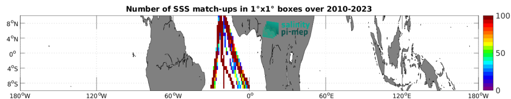
Figure 5: Number of SSS match-ups between TSG (Polarstern) SSS and the SMOS SSS L4 OI v346 - Weekly (CMEMS-CATDS-LOPS) SSS product for the Equatorial Ocean 10N-10S Pi-MEP region over 1^\circ \times 1^\circ boxes and for the full satellite product period.
