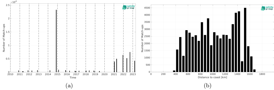
Figure 2: Number of match-ups between TSG (Polarstern) and SMOS SSS L4 OI v346 - Weekly (CMEMS-CATDS-LOPS) SSS as a function of time (a) and as function of the distance to coast (b) over the Equatorial Ocean 10N-10S Pi-MEP region and for the full satellite product period.
