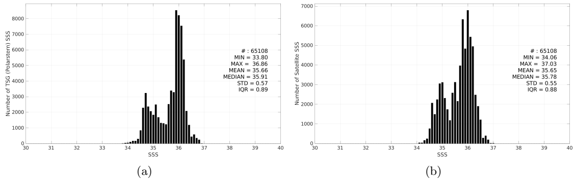
Figure 3: Histograms of SSS from TSG (Polarstern) (a) and SMOS SSS L4 OI v346 - Weekly (CMEMS-CATDS-LOPS) (b) considering all match-up pairs per bins of 0.1 over the Equatorial Ocean 10N-10S Pi-MEP region and for the full satellite product period.
