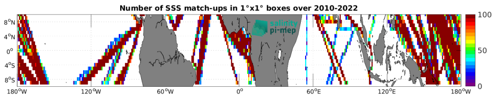
Figure 5: Number of SSS match-ups between TSG (LEGOS-DM) SSS and the SMOS SSS L4 OI v346 - Weekly (CMEMS-CATDS-LOPS) SSS product for the Equatorial Ocean 10N-10S Pi-MEP region over 1^\circ \times 1^\circ boxes and for the full satellite product period.
