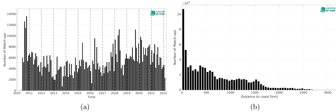
Figure 2: Number of match-ups between TSG (LEGOS-DM) and SMOS SSS L4 OI v346 - Weekly (CMEMS-CATDS-LOPS) SSS as a function of time (a) and as function of the distance to coast (b) over the Equatorial Ocean 10N-10S Pi-MEP region and for the full satellite product period.
