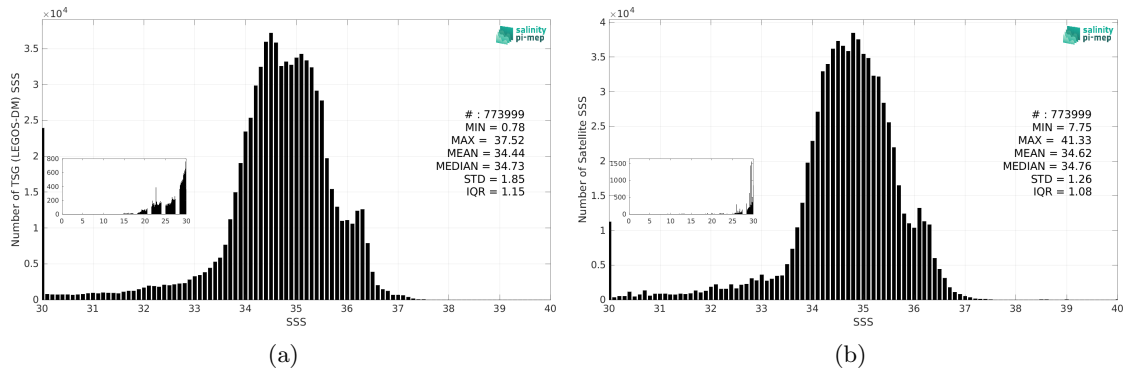
Figure 3: Histograms of SSS from TSG (LEGOS-DM) (a) and SMOS SSS L4 OI v346 - Weekly (CMEMS-CATDS-LOPS) (b) considering all match-up pairs per bins of 0.1 over the Equatorial Ocean 10N-10S Pi-MEP region and for the full satellite product period.
