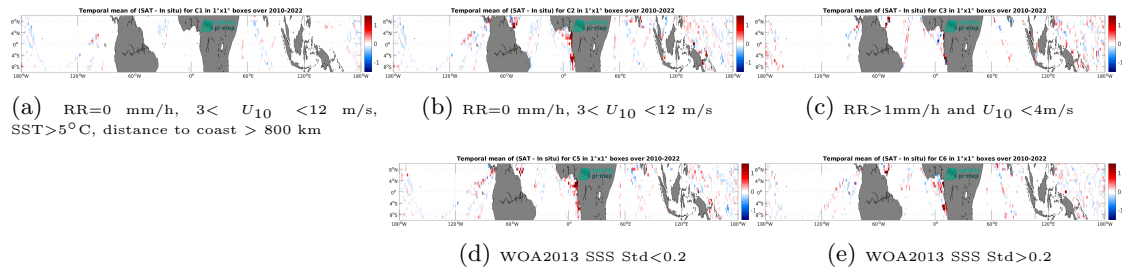
Figure 14: Temporal mean gridded over spatial boxes of size 1^\circ \times 1^\circ of \Delta\text{SSS} (SMOS SSS L4 OI v346 - Weekly (CMEMS-CATDS-LOPS) - TSG (LEGOS-DM)) for 5 different subdatasets corresponding to: RR=0 mm/h, 3 < U_{10} < 12 m/s, SST>5°C, distance to coast > 800 km (a), RR=0 mm/h, 3 < U_{10} < 12 m/s (b), RR>1mm/h and U_{10} < 4 m/s (c), WOA2013 SSS Std<0.2 (d), WOA2013 SSS Std>0.2 (e).
