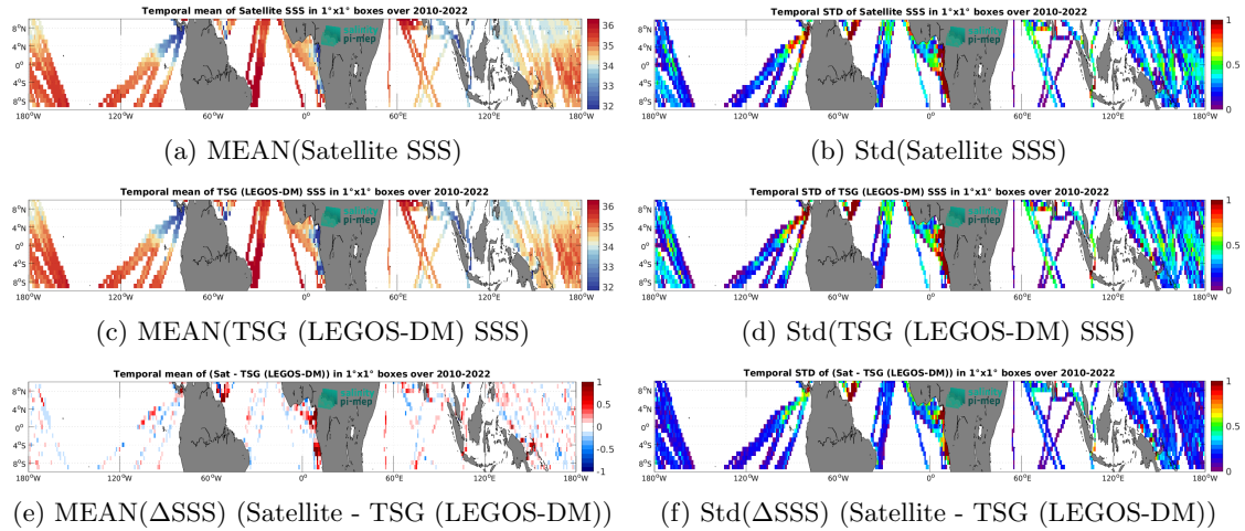
Figure 7: Temporal mean (left) and Std (right) of SSS from SMOS SSS L4 OI v346 - Weekly (CMEMS-CATDS-LOPS) (top), TSG (LEGOS-DM) (middle), and of \Delta SSS (Satellite - TSG (LEGOS-DM)). Only match-up pairs are used to generate these maps.
