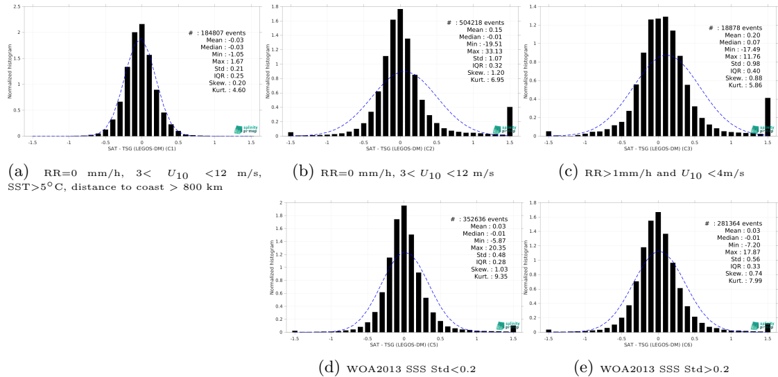
Figure 15: Normalized histogram of \Delta\text{SSS} (SMOS SSS L4 OI v346 - Weekly (CMEMS-CATDS-LOPS) - TSG (LEGOS-DM)) for 5 different subdatasets corresponding to: RR=0 mm/h, 3 < U_{10} < 12 m/s, SST>5°C, distance to coast > 800 km (a), RR=0 mm/h, 3 < U_{10} < 12 m/s (b), RR>1mm/h and U_{10} < 4 m/s (c), WOA2013 SSS Std<0.2 (d), WOA2013 SSS Std>0.2 (e).
