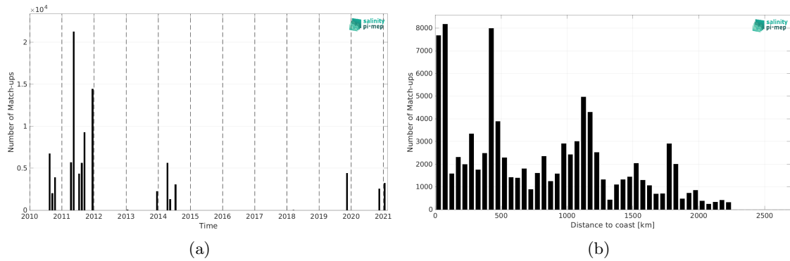
Figure 2: Number of match-ups between TSG (GOSUD-Sailing-ship) and SMOS SSS L4 OI v346 - Weekly (CMEMS-CATDS-LOPS) SSS as a function of time (a) and as function of the distance to coast (b) over the Equatorial Ocean 10N-10S Pi-MEP region and for the full satellite product period.
