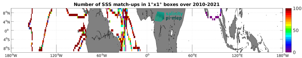
Figure 5: Number of SSS match-ups between TSG (GOSUD-Sailing-ship) SSS and the SMOS SSS L4 OI v346 - Weekly (CMEMS-CATDS-LOPS) SSS product for the Equatorial Ocean 10N-10S Pi-MEP region over 1^\circ \times 1^\circ boxes and for the full satellite product period.
