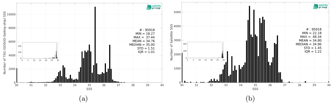
Figure 3: Histograms of SSS from TSG (GOSUD-Sailing-ship) (a) and SMOS SSS L4 OI v346 - Weekly (CMEMS-CATDS-LOPS) (b) considering all match-up pairs per bins of 0.1 over the Equatorial Ocean 10N-10S Pi-MEP region and for the full satellite product period.
