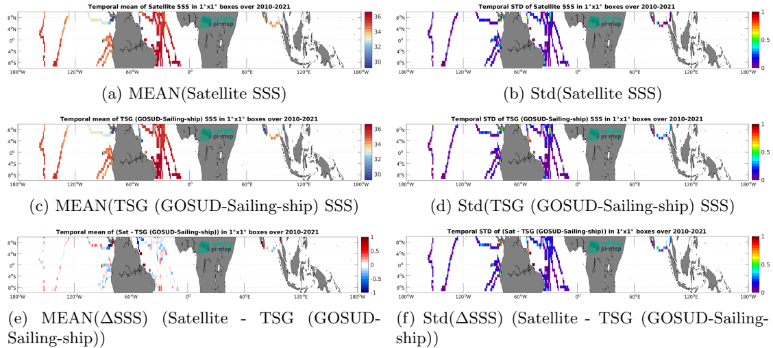
Figure 7: Temporal mean (left) and Std (right) of SSS from SMOS SSS L4 OI v346 - Weekly (CMEMS-CATDS-LOPS) (top), TSG (GOSUD-Sailing-ship) (middle), and of \Delta SSS (Satellite - TSG (GOSUD-Sailing-ship)). Only match-up pairs are used to generate these maps.
