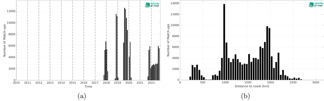
Figure 2: Number of match-ups between Saildrone and SMOS SSS L4 OI v346 - Weekly (CMEMS-CATDS-LOPS) SSS as a function of time (a) and as function of the distance to coast (b) over the Equatorial Ocean 10N-10S Pi-MEP region and for the full satellite product period.
