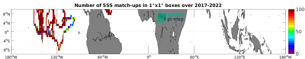
Figure 5: Number of SSS match-ups between Saildrone SSS and the SMOS SSS L4 OI v346 - Weekly (CMEMS-CATDS-LOPS) SSS product for the Equatorial Ocean 10N-10S Pi-MEP region over 1^\circ \times 1^\circ boxes and for the full satellite product period.
