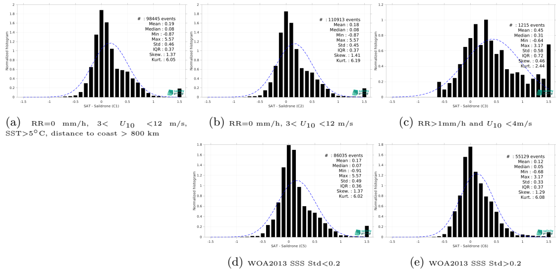
Figure 15: Normalized histogram of \Delta SSS (SMOS SSS L4 OI v346 - Weekly (CMEMS-CATDS-LOPS) - Saildrone) for 5 different subdatasets corresponding to: RR=0 mm/h, 3 < U_{10} < 12 m/s, SST>5°C, distance to coast > 800 km (a), RR=0 mm/h, 3 < U_{10} < 12 m/s (b), RR>1mm/h and U_{10} < 4 m/s (c), WOA2013 SSS Std<0.2 (d), WOA2013 SSS Std>0.2 (e).
