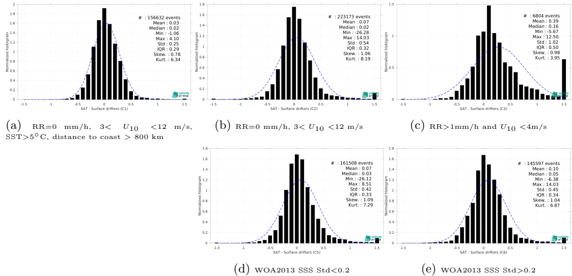
Figure 14: Normalized histogram of \Delta SSS (SMOS SSS L4 OI v346 - Weekly (CMEMS-CATDS-LOPS) - Surface drifters) for 5 different subdatasets corresponding to: RR=0 mm/h, 3 < U_{10} < 12 m/s, SST >5^\circ\text{C} , distance to coast > 800 km (a), RR=0 mm/h, 3 < U_{10} < 12 m/s (b), RR >1 mm/h and U_{10} < 4 m/s (c), WOA2013 SSS Std <0.2 (d), WOA2013 SSS Std >0.2 (e).
