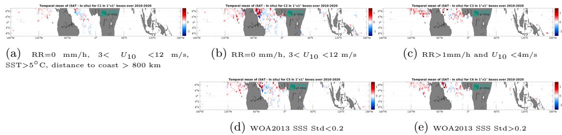
Figure 13: Temporal mean gridded over spatial boxes of size 1^\circ \times 1^\circ of \Delta SSS (SMOS SSS L4 OI v346 - Weekly (CMEMS-CATDS-LOPS) - Surface drifters) for 5 different subdatasets corresponding to:RR=0 mm/h, 3 < U_{10} < 12 m/s, SST >5^\circ\text{C} , distance to coast > 800 km (a), RR=0 mm/h, 3 < U_{10} < 12 m/s (b), RR >1 mm/h and U_{10} < 4 m/s (c), WOA2013 SSS Std <0.2 (d), WOA2013 SSS Std >0.2 (e).
