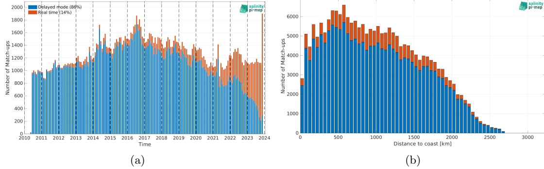
Figure 2: Number of match-ups between Argo and SMOS SSS L4 OI v346 - Weekly (CMEMS-CATDS-LOPS) SSS as a function of time (a) and as function of the distance to coast (b) over the Equatorial Ocean 10N-10S Pi-MEP region and for the full satellite product period.
