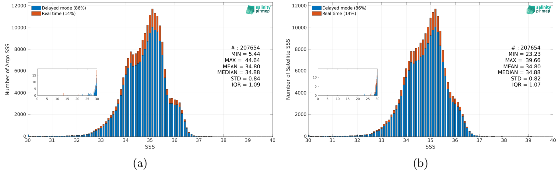
Figure 3: Histograms of SSS from Argo (a) and SMOS SSS L4 OI v346 - Weekly (CMEMS-CATDS-LOPS) (b) considering all match-up pairs per bins of 0.1 over the Equatorial Ocean 10N-10S Pi-MEP region and for the full satellite product period.
