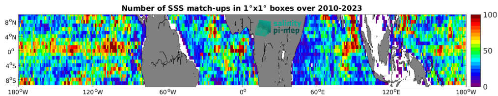
Figure 5: Number of SSS match-ups between Argo SSS and the SMOS SSS L4 OI v346 - Weekly (CMEMS-CATDS-LOPS) SSS product for the Equatorial Ocean 10N-10S Pi-MEP region over 1^\circ \times 1^\circ boxes and for the full satellite product period.
