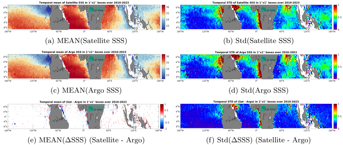
Figure 7: Temporal mean (left) and Std (right) of SSS from SMOS SSS L4 OI v346 - Weekly (CMEMS-CATDS-LOPS) (top), Argo (middle), and of \Delta SSS (Satellite - Argo). Only match-up pairs are used to generate these maps.
