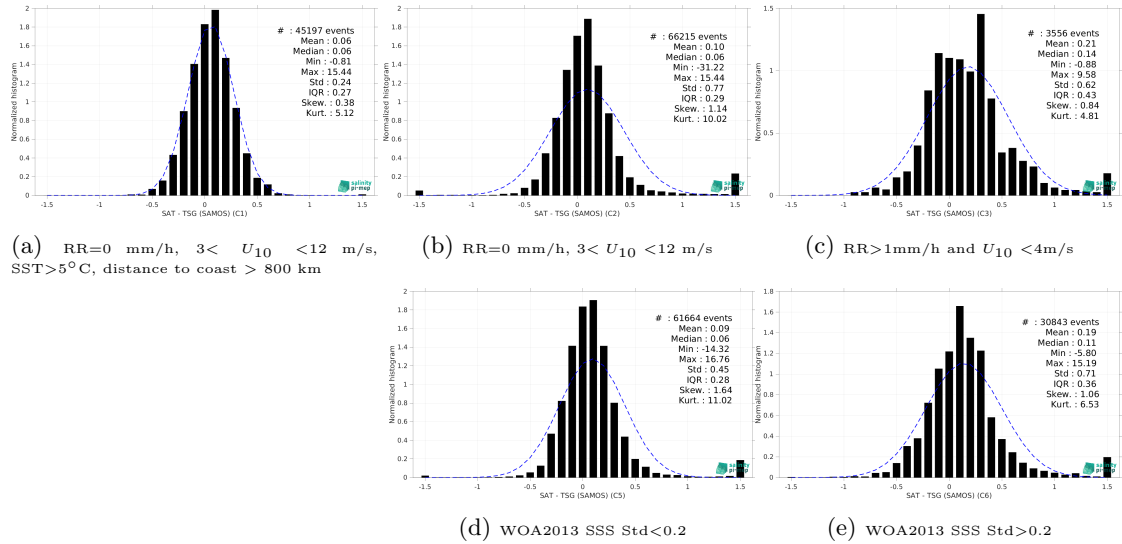
Figure 13: Normalized histogram of \Delta SSS (SMOS SSS L4 OI v342 - Weekly (CMEMS-CATDS-LOPS) - TSG (SAMOS)) for 5 different subdatasets corresponding to: RR=0 mm/h, 3 < U_{10} < 12 m/s, SST >5^\circ C, distance to coast > 800 km (a), RR=0 mm/h, 3 < U_{10} < 12 m/s (b), RR >1 mm/h and U_{10} < 4 m/s (c), WOA2013 SSS Std <0.2 (d), WOA2013 SSS Std >0.2 (e).
