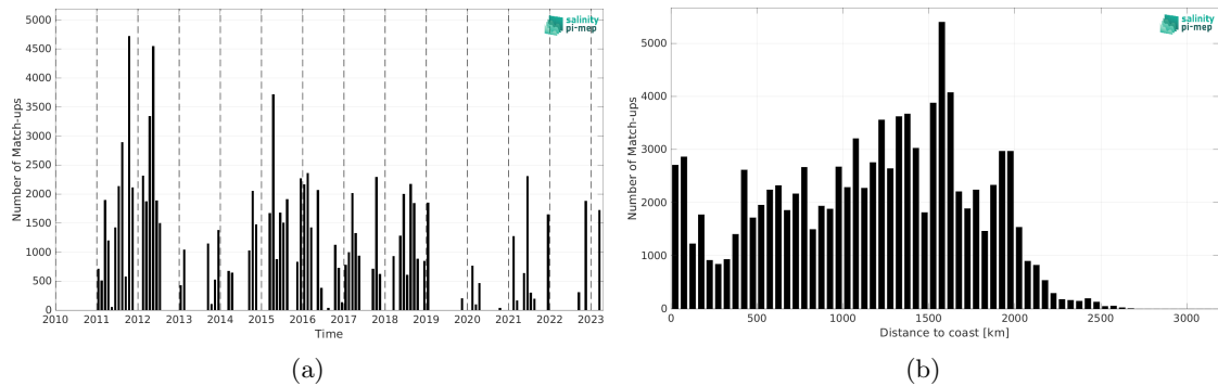
Figure 1: Number of match-ups between TSG (SAMOS) and SMOS SSS L4 OI v342 - Weekly (CMEMS-CATDS-LOPS) SSS as a function of time (a) and as function of the distance to coast (b) over the Equatorial Ocean 10N-10S Pi-MEP region and for the full satellite product period.
