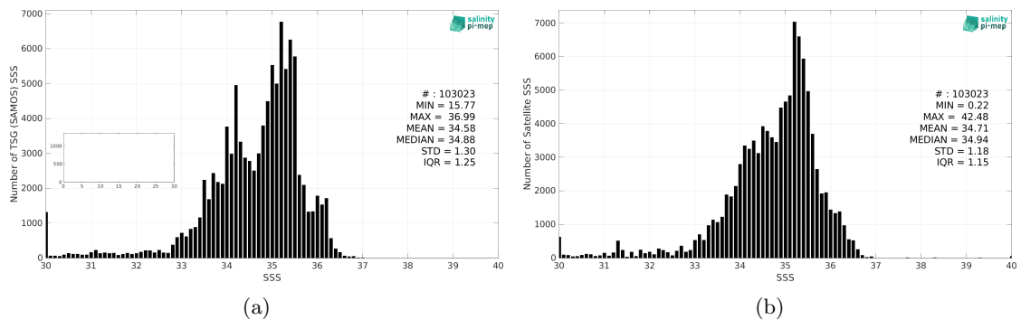
Figure 2: Histograms of SSS from TSG (SAMOS) (a) and SMOS SSS L4 OI v342 - Weekly (CMEMS-CATDS-LOPS) (b) considering all match-up pairs per bins of 0.1 over the Equatorial Ocean 10N-10S Pi-MEP region and for the full satellite product period.
