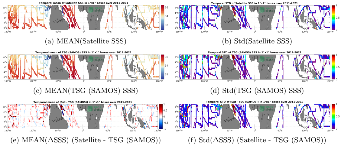
Figure 6: Temporal mean (left) and Std (right) of SSS from SMOS SSS L4 OI v342 - Weekly (CMEMS-CATDS-LOPS) (top), TSG (SAMOS) (middle), and of \Delta SSS (Satellite - TSG (SAMOS)). Only match-up pairs are used to generate these maps.
