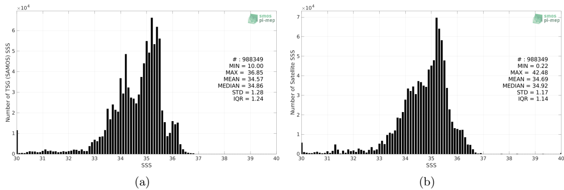
Figure 2: Histograms of SSS from TSG (SAMOS) (a) and SMOS SSS L4 OI v342 - Weekly (CMEMS-CATDS-LOPS) (b) considering all match-up pairs per bins of 0.1 over the Equatorial Ocean 10N-10S Pi-MEP region and for the full satellite product period.
