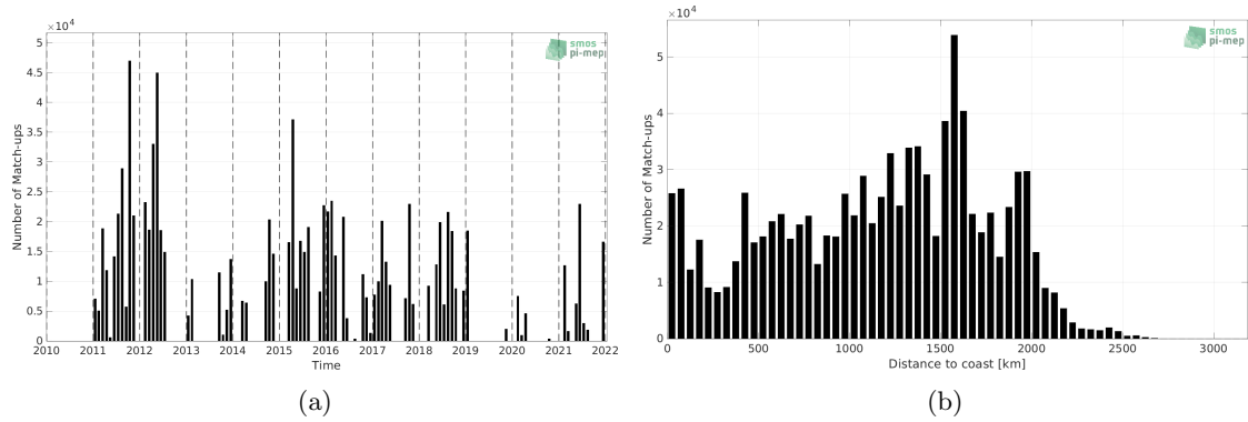
Figure 1: Number of match-ups between TSG (SAMOS) and SMOS SSS L4 OI v342 - Weekly (CMEMS-CATDS-LOPS) SSS as a function of time (a) and as function of the distance to coast (b) over the Equatorial Ocean 10N-10S Pi-MEP region and for the full satellite product period.
