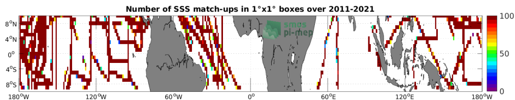
Figure 4: Number of SSS match-ups between TSG (SAMOS) SSS and the SMOS SSS L4 OI v342 - Weekly (CMEMS-CATDS-LOPS) SSS product for the Equatorial Ocean 10N-10S Pi-MEP region over 1^\circ \times 1^\circ boxes and for the full satellite product period.
