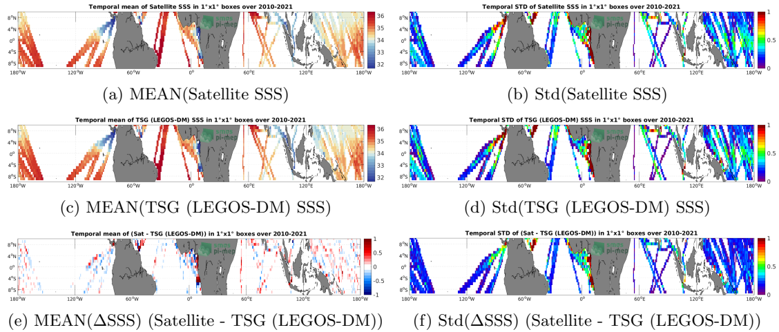
Figure 6: Temporal mean (left) and Std (right) of SSS from SMOS SSS L4 OI v342 - Weekly (CMEMS-CATDS-LOPS) (top), TSG (LEGOS-DM) (middle), and of \Delta SSS (Satellite - TSG (LEGOS-DM)). Only match-up pairs are used to generate these maps.
