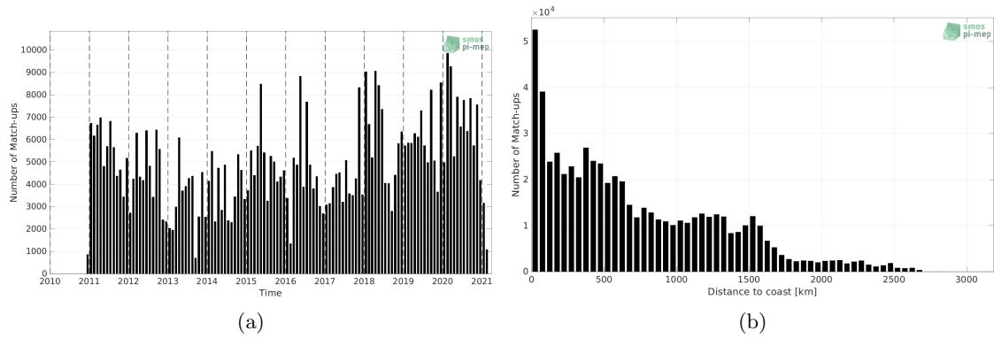
Figure 1: Number of match-ups between TSG (LEGOS-DM) and SMOS SSS L4 OI v342 - Weekly (CMEMS-CATDS-LOPS) SSS as a function of time (a) and as function of the distance to coast (b) over the Equatorial Ocean 10N-10S Pi-MEP region and for the full satellite product period.
