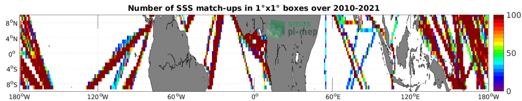
Figure 4: Number of SSS match-ups between TSG (LEGOS-DM) SSS and the SMOS SSS L4 OI v342 - Weekly (CMEMS-CATDS-LOPS) SSS product for the Equatorial Ocean 10N-10S Pi-MEP region over 1^\circ \times 1^\circ boxes and for the full satellite product period.
