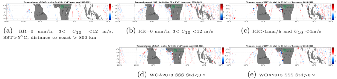
Figure 12: Temporal mean gridded over spatial boxes of size 1^{\circ}\times 1^{\circ} of \Delta\text{SSS} (SMOS SSS L4 OI v342 - Weekly (CMEMS-CATDS-LOPS) - TSG (LEGOS-DM)) for 5 different subdatasets corresponding to:RR=0 mm/h, 3 < U_{10} < 12 m/s, SST >5^{\circ}\text{C} , distance to coast > 800 km (a), RR=0 mm/h, 3 < U_{10} < 12 m/s (b), RR >1 mm/h and U_{10} < 4 m/s (c), WOA2013 SSS Std <0.2 (d), WOA2013 SSS Std >0.2 (e).
