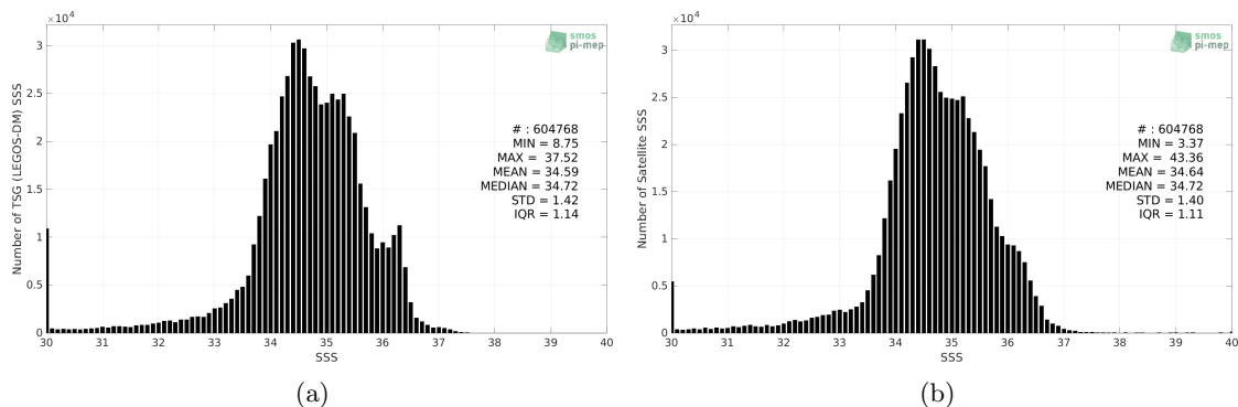
Figure 2: Histograms of SSS from TSG (LEGOS-DM) (a) and SMOS SSS L4 OI v342 - Weekly (CMEMS-CATDS-LOPS) (b) considering all match-up pairs per bins of 0.1 over the Equatorial Ocean 10N-10S Pi-MEP region and for the full satellite product period.
