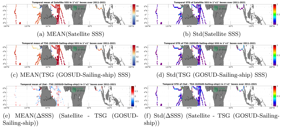
Figure 6: Temporal mean (left) and Std (right) of SSS from SMOS SSS L4 OI v342 - Weekly (CMEMS-CATDS-LOPS) (top), TSG (GOSUD-Sailing-ship) (middle), and of \Delta SSS (Satellite - TSG (GOSUD-Sailing-ship)). Only match-up pairs are used to generate these maps.
