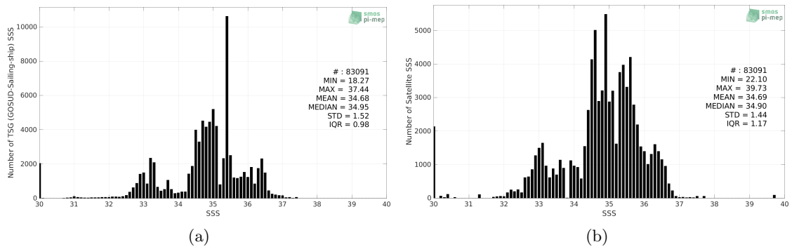
Figure 2: Histograms of SSS from TSG (GOSUD-Sailing-ship) (a) and SMOS SSS L4 OI v342 - Weekly (CMEMS-CATDS-LOPS) (b) considering all match-up pairs per bins of 0.1 over the Equatorial Ocean 10N-10S Pi-MEP region and for the full satellite product period.
