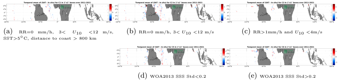
Figure 12: Temporal mean gridded over spatial boxes of size 1^{\circ}\times 1^{\circ} of \Delta SSS (SMOS SSS L4 OI v342 - Weekly (CMEMS-CATDS-LOPS) - TSG (GOSUD-Sailing-ship)) for 5 different sub-datasets corresponding to:RR=0 mm/h, 3 < U_{10} < 12 m/s, SST >5^{\circ}\text{C} , distance to coast > 800 km (a), RR=0 mm/h, 3 < U_{10} < 12 m/s (b), RR >1 mm/h and U_{10} < 4 m/s (c), WOA2013 SSS Std <0.2 (d), WOA2013 SSS Std >0.2 (e).
