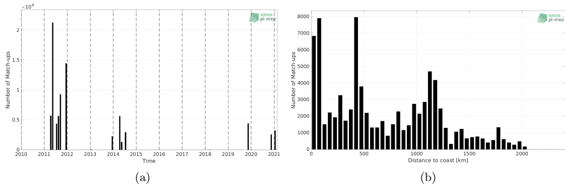
Figure 1: Number of match-ups between TSG (GOSUD-Sailing-ship) and SMOS SSS L4 OI v342 - Weekly (CMEMS-CATDS-LOPS) SSS as a function of time (a) and as function of the distance to coast (b) over the Equatorial Ocean 10N-10S Pi-MEP region and for the full satellite product period.
