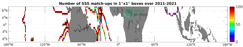
Figure 4: Number of SSS match-ups between TSG (GOSUD-Sailing-ship) SSS and the SMOS SSS L4 OI v342 - Weekly (CMEMS-CATDS-LOPS) SSS product for the Equatorial Ocean 10N-10S Pi-MEP region over 1^\circ \times 1^\circ boxes and for the full satellite product period.
