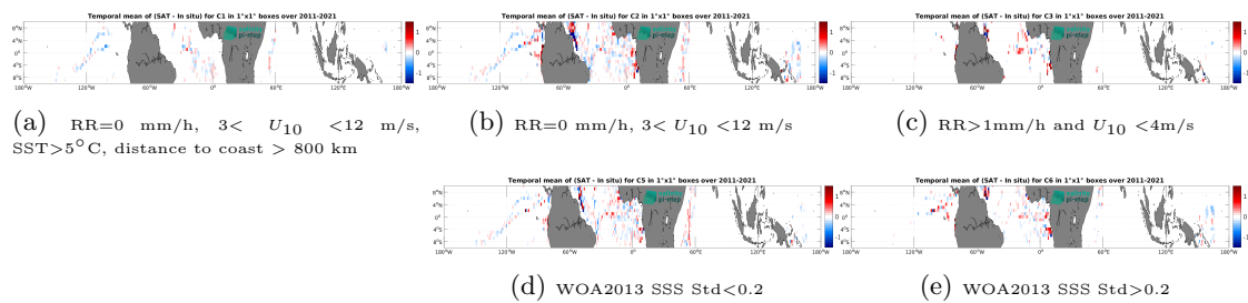
Figure 12: Temporal mean gridded over spatial boxes of size 1^\circ \times 1^\circ of \Delta SSS (SMOS SSS L4 OI v342 - Weekly (CMEMS-CATDS-LOPS) - TSG (GOSUD-Research-vessel)) for 5 different subdatasets corresponding to:RR=0 mm/h, 3 < U_{10} < 12 m/s, SST>5°C, distance to coast > 800 km (a), RR=0 mm/h, 3 < U_{10} < 12 m/s (b), RR>1mm/h and U_{10} < 4 m/s (c), WOA2013 SSS Std<0.2 (d), WOA2013 SSS Std>0.2 (e).
