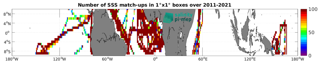
Figure 4: Number of SSS match-ups between TSG (GOSUD-Research-vessel) SSS and the SMOS SSS L4 OI v342 - Weekly (CMEMS-CATDS-LOPS) SSS product for the Equatorial Ocean 10N-10S Pi-MEP region over 1^\circ \times 1^\circ boxes and for the full satellite product period.
