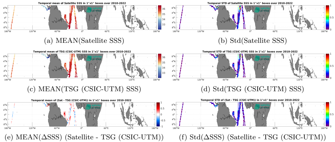
Figure 6: Temporal mean (left) and Std (right) of SSS from SMOS SSS L4 OI v342 - Weekly (CMEMS-CATDS-LOPS) (top), TSG (CSIC-UTM) (middle), and of \Delta SSS (Satellite - TSG (CSIC-UTM)). Only match-up pairs are used to generate these maps.
