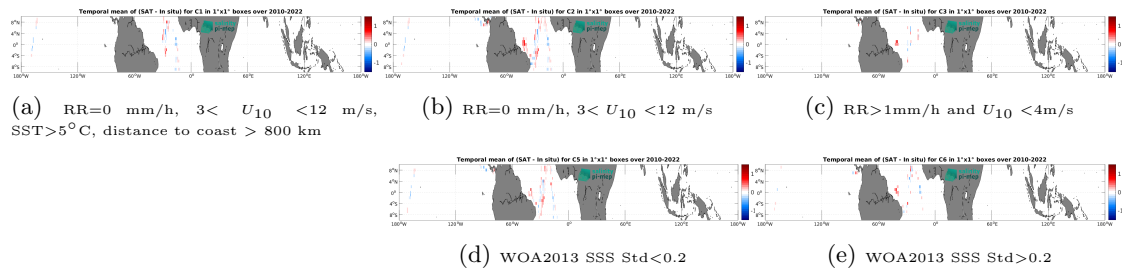
Figure 12: Temporal mean gridded over spatial boxes of size 1^\circ \times 1^\circ of \Delta SSS (SMOS SSS L4 OI v342 - Weekly (CMEMS-CATDS-LOPS) - TSG (CSIC-UTM)) for 5 different subdatasets corresponding to: RR=0 mm/h, 3 < U_{10} < 12 m/s, SST >5^\circ\text{C} , distance to coast > 800 km (a), RR=0 mm/h, 3 < U_{10} < 12 m/s (b), RR >1 mm/h and U_{10} < 4 m/s (c), WOA2013 SSS Std <0.2 (d), WOA2013 SSS Std >0.2 (e).
