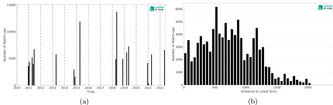
Figure 1: Number of match-ups between TSG (CSIC-UTM) and SMOS SSS L4 OI v342 - Weekly (CMEMS-CATDS-LOPS) SSS as a function of time (a) and as function of the distance to coast (b) over the Equatorial Ocean 10N-10S Pi-MEP region and for the full satellite product period.
