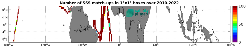
Figure 4: Number of SSS match-ups between TSG (CSIC-UTM) SSS and the SMOS SSS L4 OI v342 - Weekly (CMEMS-CATDS-LOPS) SSS product for the Equatorial Ocean 10N-10S Pi-MEP region over 1^\circ \times 1^\circ boxes and for the full satellite product period.
