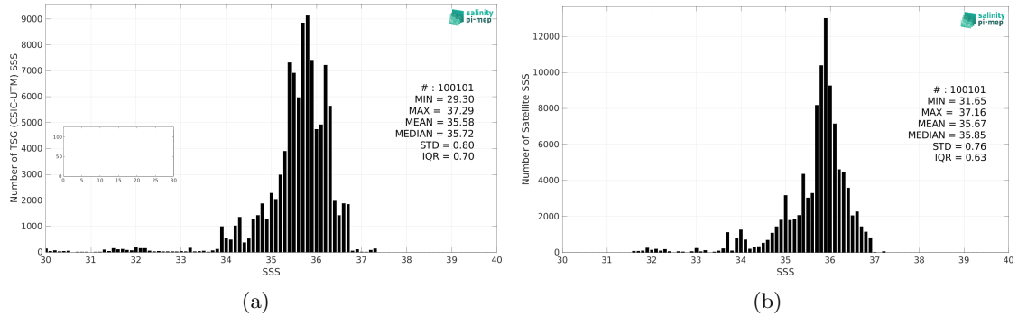
Figure 2: Histograms of SSS from TSG (CSIC-UTM) (a) and SMOS SSS L4 OI v342 - Weekly (CMEMS-CATDS-LOPS) (b) considering all match-up pairs per bins of 0.1 over the Equatorial Ocean 10N-10S Pi-MEP region and for the full satellite product period.
