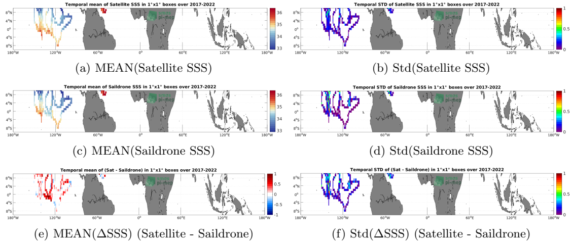
Figure 6: Temporal mean (left) and Std (right) of SSS from SMOS SSS L4 OI v342 - Weekly (CMEMS-CATDS-LOPS) (top), Saildrone (middle), and of \Delta SSS (Satellite - Saildrone). Only match-up pairs are used to generate these maps.
