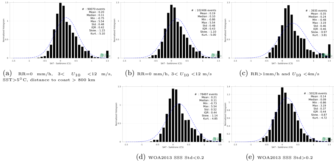
Figure 13: Normalized histogram of \Delta SSS (SMOS SSS L4 OI v342 - Weekly (CMEMS-CATDS-LOPS) - Saldrone) for 5 different subdatasets corresponding to: RR=0 mm/h, 3 < U_{10} < 12 m/s, SST>5°C, distance to coast > 800 km (a), RR=0 mm/h, 3 < U_{10} < 12 m/s (b), RR>1mm/h and U_{10} < 4 m/s (c), WOA2013 SSS Std<0.2 (d), WOA2013 SSS Std>0.2 (e).
