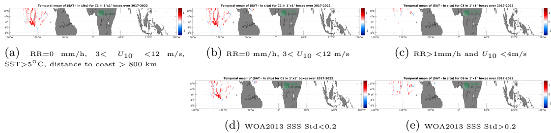
Figure 12: Temporal mean gridded over spatial boxes of size 1^\circ \times 1^\circ of \Delta SSS (SMOS SSS L4 OI v342 - Weekly (CMEMS-CATDS-LOPS) - Saldrone) for 5 different subdatasets corresponding to: RR=0 mm/h, 3 < U_{10} < 12 m/s, SST>5°C, distance to coast > 800 km (a), RR=0 mm/h, 3 < U_{10} < 12 m/s (b), RR>1mm/h and U_{10} < 4 m/s (c), WOA2013 SSS Std<0.2 (d), WOA2013 SSS Std>0.2 (e).
