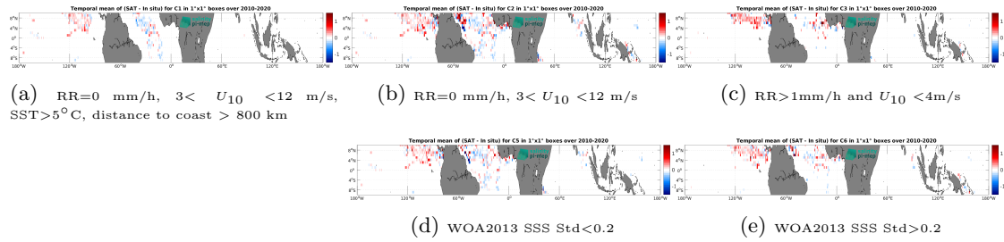
Figure 11: Temporal mean gridded over spatial boxes of size 1^\circ \times 1^\circ of \Delta SSS (SMOS SSS L4 OI v342 - Weekly (CMEMS-CATDS-LOPS) - Surface drifters) for 5 different subdatasets corresponding to:RR=0 mm/h, 3 < U_{10} < 12 m/s, SST >5^\circ C, distance to coast > 800 km (a), RR=0 mm/h, 3 < U_{10} < 12 m/s (b), RR >1 mm/h and U_{10} < 4 m/s (c), WOA2013 SSS Std <0.2 (d), WOA2013 SSS Std >0.2 (e).
