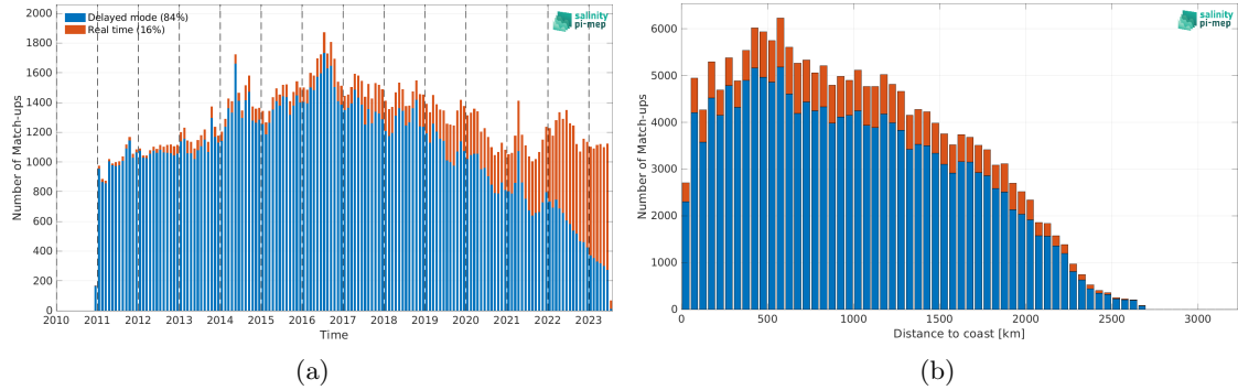
Figure 1: Number of match-ups between Argo and SMOS SSS L4 OI v342 - Weekly (CMEMS-CATDS-LOPS) SSS as a function of time (a) and as function of the distance to coast (b) over the Equatorial Ocean 10N-10S Pi-MEP region and for the full satellite product period.
