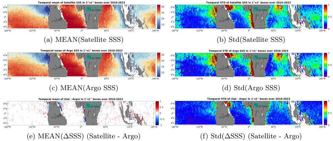
Figure 6: Temporal mean (left) and Std (right) of SSS from SMOS SSS L4 OI v342 - Weekly (CMEMS-CATDS-LOPS) (top), Argo (middle), and of \Delta SSS (Satellite - Argo). Only match-up pairs are used to generate these maps.
