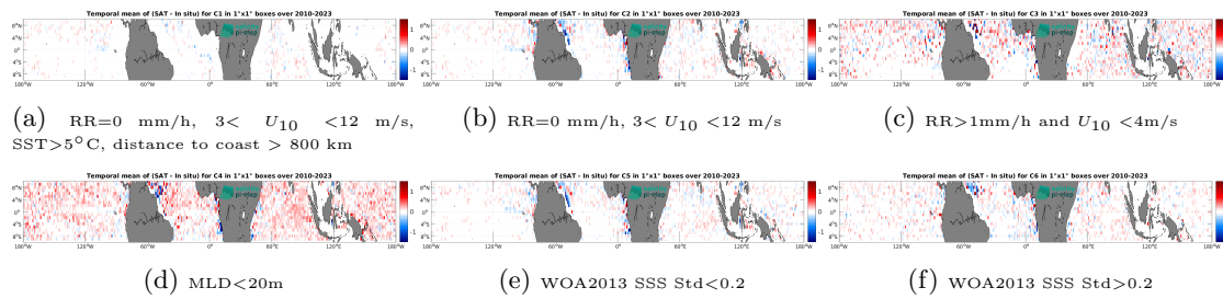
Figure 12: Temporal mean gridded over spatial boxes of size 1^\circ \times 1^\circ of \Delta SSS (SMOS SSS L4 OI v342 - Weekly (CMEMS-CATDS-LOPS) - Argo) for 6 different subdatasets corresponding to:RR=0 mm/h, 3 < U_{10} < 12 m/s, SST >5^\circ C, distance to coast > 800 km (a), RR=0 mm/h, 3 < U_{10} < 12 m/s (b), RR >1 mm/h and U_{10} < 4 m/s (c),MLD <20 m (d),WOA2013 SSS Std <0.2 (e),WOA2013 SSS Std >0.2 (f).
