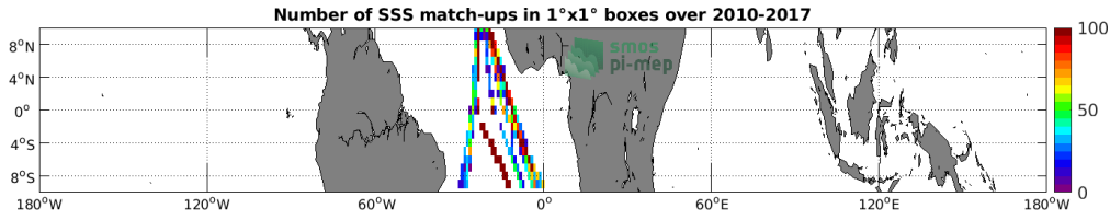
Figure 4: Number of SSS match-ups between TSG (Polarstern) SSS and the SMOS L4 v2 Weekly (CATDS-CECOS-IFREMER) SSS product for the Equatorial Ocean 10N-10S Pi-MEP region over 1^\circ \times 1^\circ boxes and for the full satellite product period.
