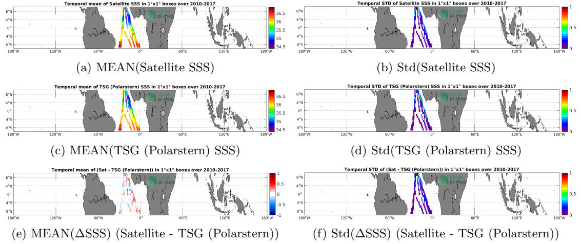
Figure 6: Temporal mean (left) and Std (right) of SSS from SMOS L4 v2 Weekly (CATDS-CECOS-IFREMER) (top), TSG (Polarstern) (middle), and of \Delta SSS (Satellite - TSG (Polarstern)). Only match-up pairs are used to generate these maps.
