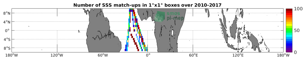
Figure 4: Number of SSS match-ups between TSG (Polarstern) SSS and the SMOS L4 v2 Weekly (CATDS-CECOS-IFREMER) SSS product for the Equatorial Ocean 10N-10S Pi-MEP region over 1^\circ \times 1^\circ boxes and for the full satellite product period.
