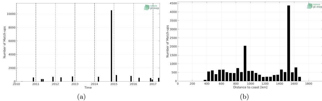
Figure 1: Number of match-ups between TSG (Polarstern) and SMOS L4 v2 Weekly (CATDS-CECOS-IFREMER) SSS as a function of time (a) and as function of the distance to coast (b) over the Equatorial Ocean 10N-10S Pi-MEP region and for the full satellite product period.
