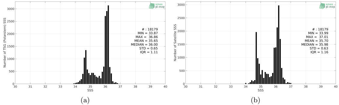
Figure 2: Histograms of SSS from TSG (Polarstern) (a) and SMOS L4 v2 Weekly (CATDS-CECOS-IFREMER) (b) considering all match-up pairs per bins of 0.1 over the Equatorial Ocean 10N-10S Pi-MEP region and for the full satellite product period.
