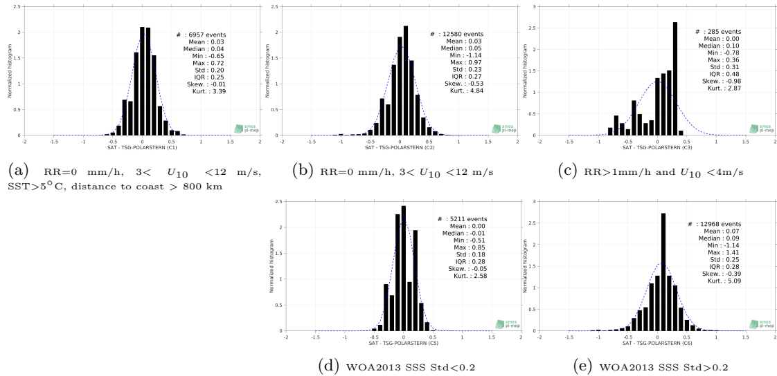
Figure 13: Normalized histogram of \Delta SSS (SMOS-L4-CATDS-CECOS-IFREMER-V2-WEEKLY-0.5DEG - TSG-POLARSTERN) for 5 different subdatasets corresponding to: RR=0 mm/h, 3 < U_{10} < 12 m/s, SST >5^\circ C, distance to coast > 800 km (a), RR=0 mm/h, 3 < U_{10} < 12 m/s (b), RR >1 mm/h and U_{10} < 4 m/s (c), WOA2013 SSS Std <0.2 (d), WOA2013 SSS Std >0.2 (e).
