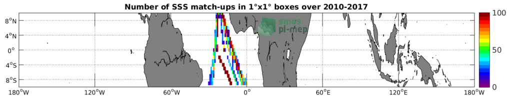
Figure 4: Number of SSS match-ups between TSG-POLARSTERN SSS and the SMOS-L4-CATDS-CECOS-IFREMER-V2-WEEKLY-0.5DEG SSS product for the Equatorial Ocean 10N-10S Pi-MEP region over 1^\circ \times 1^\circ boxes and for the full satellite product period.
