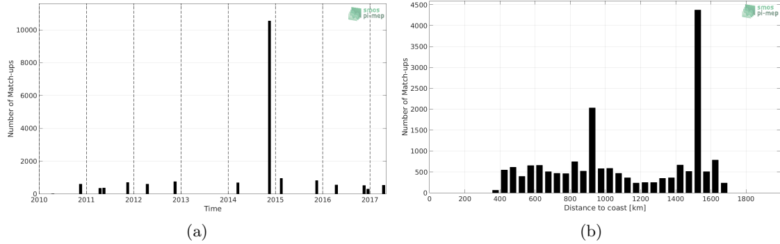
Figure 1: Number of match-ups between TSG-POLARSTERN and SMOS-L4-CATDS-CECOS-IFREMER-V2-WEEKLY-0.5DEG SSS as a function of time (a) and as function of the distance to coast (b) over the Equatorial Ocean 10N-10S Pi-MEP region and for the full satellite product period.
