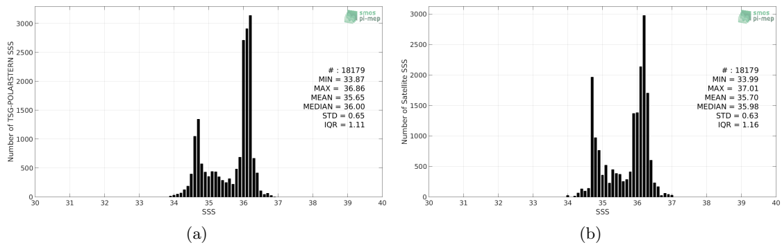
Figure 2: Histograms of SSS from TSG-POLARSTERN (a) and SMOS-L4-CATDS-CECOS-IFREMER-V2-WEEKLY-0.5DEG (b) considering all match-up pairs per bins of 0.1 over the Equatorial Ocean 10N-10S Pi-MEP region and for the full satellite product period.
