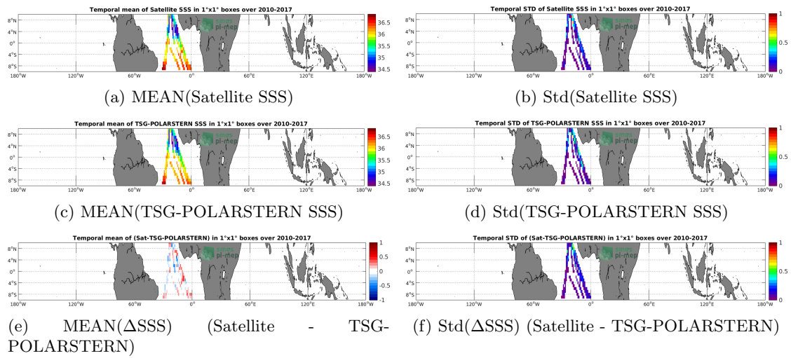
Figure 6: Temporal mean (left) and Std (right) of SSS from SMOS-L4-CATDS-CECOS-IFREMER-V2-WEEKLY-0.5DEG (top), TSG-POLARSTERN (middle), and of \Delta SSS (Satellite - TSG-POLARSTERN). Only match-up pairs are used to generate these maps.
