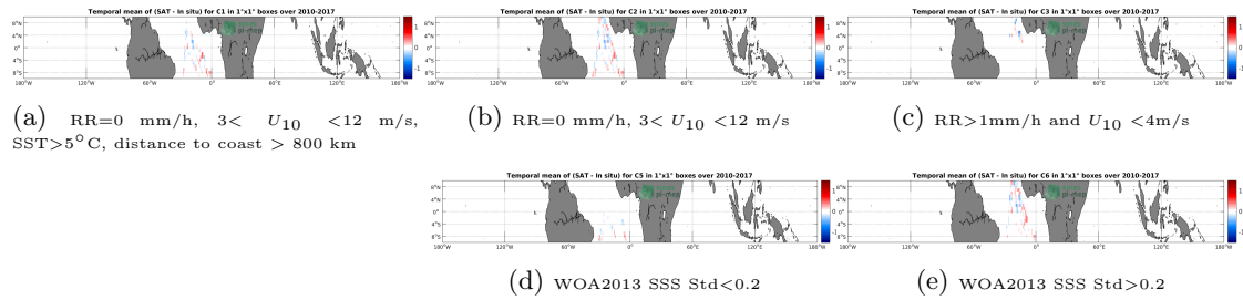
Figure 12: Temporal mean gridded over spatial boxes of size 1^\circ \times 1^\circ of \Delta SSS (SMOS-L4-CATDS-CECOS-IFREMER-V2-WEEKLY-0.5DEG - TSG-POLARSTERN) for 5 different subdatasets corresponding to:RR=0 mm/h, 3 < U_{10} < 12 m/s, SST >5^\circ C, distance to coast > 800 km (a), RR=0 mm/h, 3 < U_{10} < 12 m/s (b), RR >1 mm/h and U_{10} < 4 m/s (c), WOA2013 SSS Std <0.2 (d), WOA2013 SSS Std >0.2 (e).
