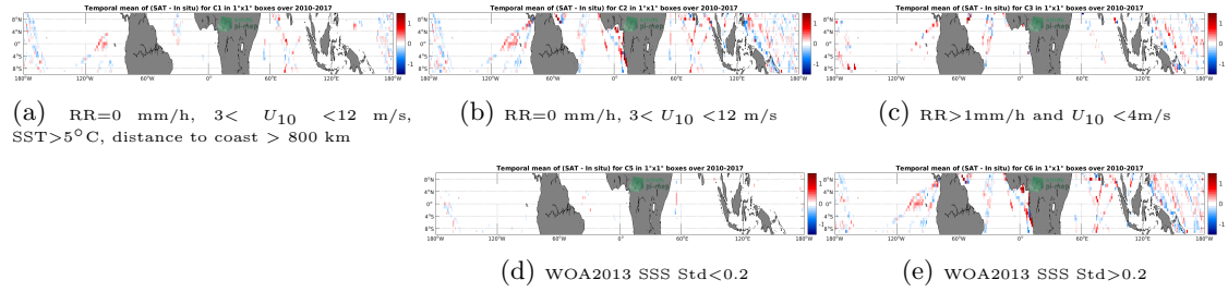
Figure 12: Temporal mean gridded over spatial boxes of size 1^{\circ}\times 1^{\circ} of \Delta\text{SSS} (SMOS L4 v2 Weekly (CATDS-CECOS-IFREMER) - TSG (LEGOS-DM)) for 5 different subdatasets corresponding to: \text{RR}=0 mm/h, 3 < U_{10} < 12 m/s, \text{SST} > 5^{\circ}\text{C} , distance to coast > 800 km (a), \text{RR}=0 mm/h, 3 < U_{10} < 12 m/s (b), \text{RR} > 1 mm/h and U_{10} < 4 m/s (c), WOA2013 SSS Std < 0.2 (d), WOA2013 SSS Std > 0.2 (e).
