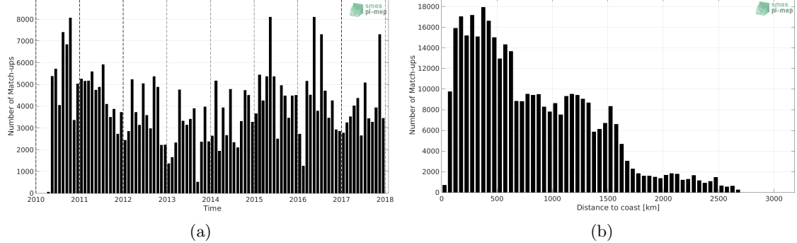
Figure 1: Number of match-ups between TSG (LEGOS-DM) and SMOS L4 v2 Weekly (CATDS-CECOS-IFREMER) SSS as a function of time (a) and as function of the distance to coast (b) over the Equatorial Ocean 10N-10S Pi-MEP region and for the full satellite product period.
