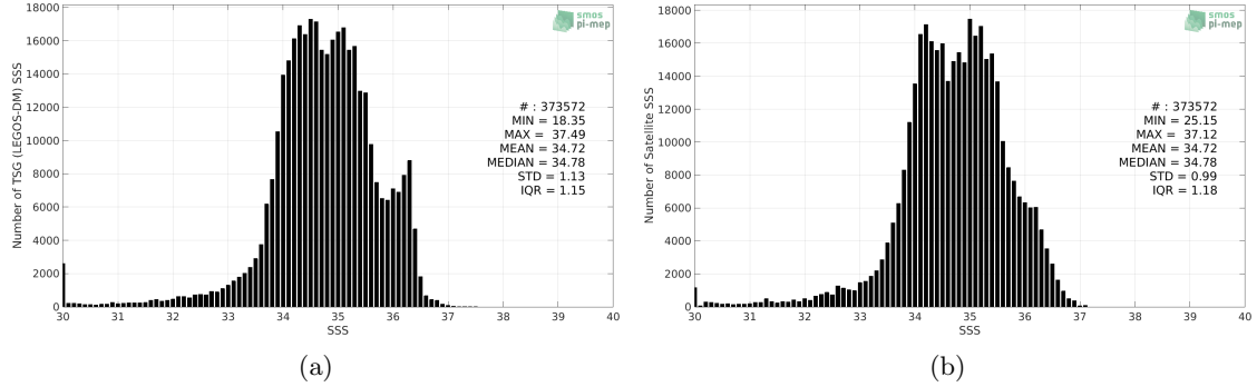
Figure 2: Histograms of SSS from TSG (LEGOS-DM) (a) and SMOS L4 v2 Weekly (CATDS-CECOS-IFREMER) (b) considering all match-up pairs per bins of 0.1 over the Equatorial Ocean 10N-10S Pi-MEP region and for the full satellite product period.
