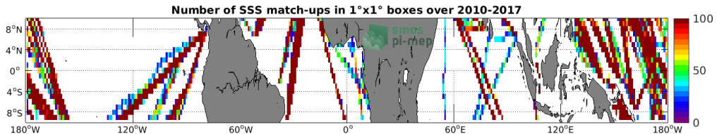
Figure 4: Number of SSS match-ups between TSG (LEGOS-DM) SSS and the SMOS L4 v2 Weekly (CATDS-CECOS-IFREMER) SSS product for the Equatorial Ocean 10N-10S Pi-MEP region over 1°x1° boxes and for the full satellite product period.
