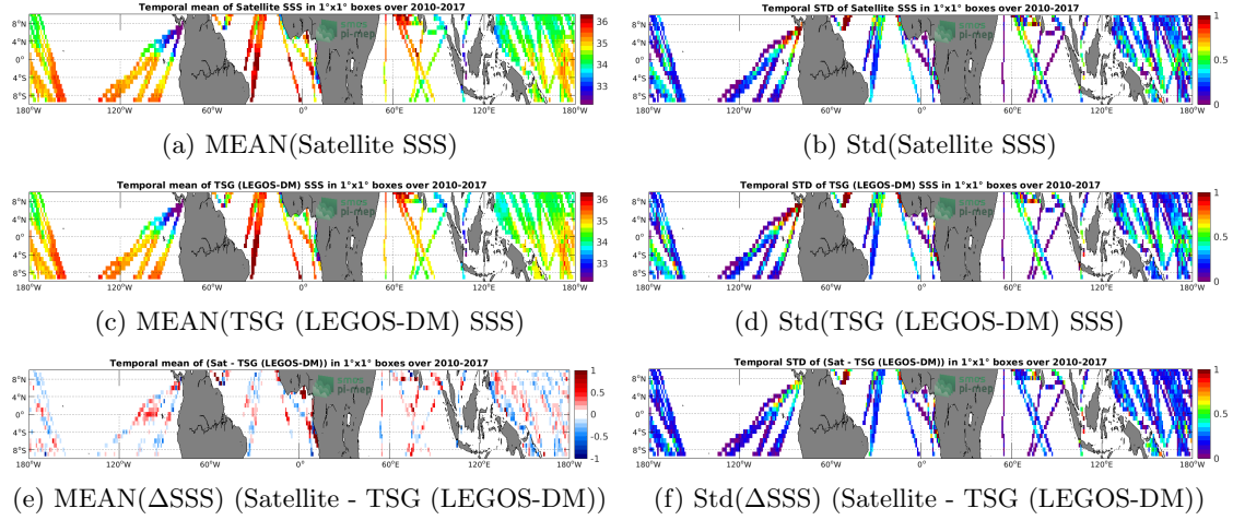
Figure 6: Temporal mean (left) and Std (right) of SSS from SMOS L4 v2 Weekly (CATDS-CECOS-IFREMER) (top), TSG (LEGOS-DM) (middle), and of \Delta SSS (Satellite - TSG (LEGOS-DM)). Only match-up pairs are used to generate these maps.
