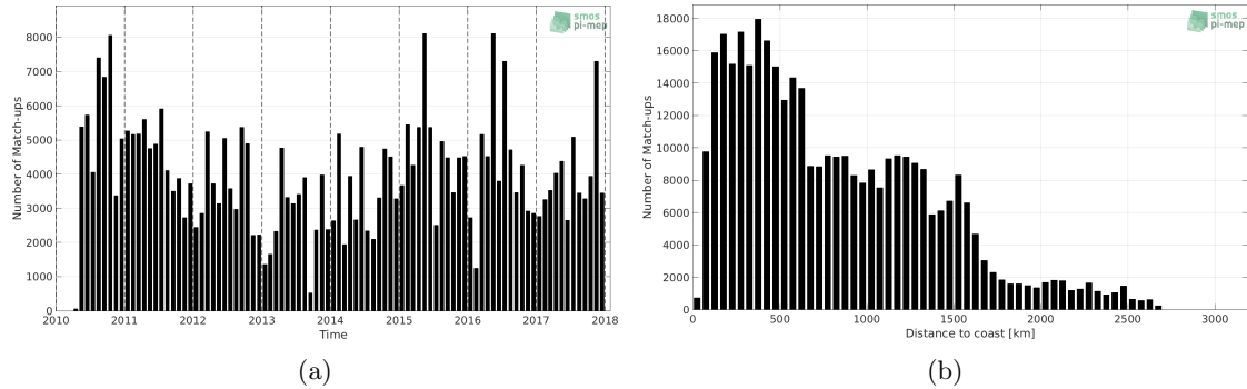
Figure 1: Number of match-ups between TSG-LEGOS-DM and SMOS-L4-CATDS-CECOS-IFREMER-V2-WEEKLY-0.5DEG SSS as a function of time (a) and as function of the distance to coast (b) over the Equatorial Ocean 10N-10S Pi-MEP region and for the full satellite product period.
