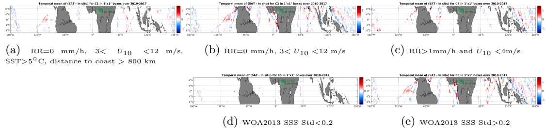
Figure 12: Temporal mean gridded over spatial boxes of size 1^{\circ}\times 1^{\circ} of \Delta\text{SSS} (SMOS-L4-CATDS-CECOS-IFREMER-V2-WEEKLY-0.5DEG - TSG-LEGOS-DM) for 5 different subdatasets corresponding to: RR=0 mm/h, 3 < U_{10} < 12 m/s, SST > 5^{\circ}\text{C} , distance to coast > 800 km (a), RR=0 mm/h, 3 < U_{10} < 12 m/s (b), RR > 1 mm/h and U_{10} < 4 m/s (c), WOA2013 SSS Std < 0.2 (d), WOA2013 SSS Std > 0.2 (e).
