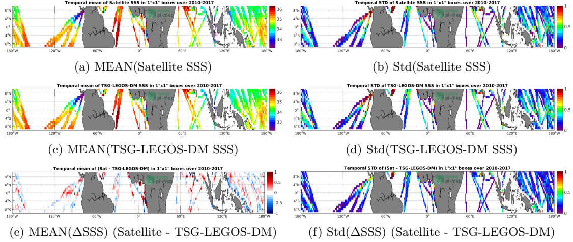
Figure 6: Temporal mean (left) and Std (right) of SSS from SMOS-L4-CATDS-CECOS-IFREMER-V2-WEEKLY-0.5DEG (top), TSG-LEGOS-DM (middle), and of \Delta SSS (Satellite - TSG-LEGOS-DM). Only match-up pairs are used to generate these maps.
