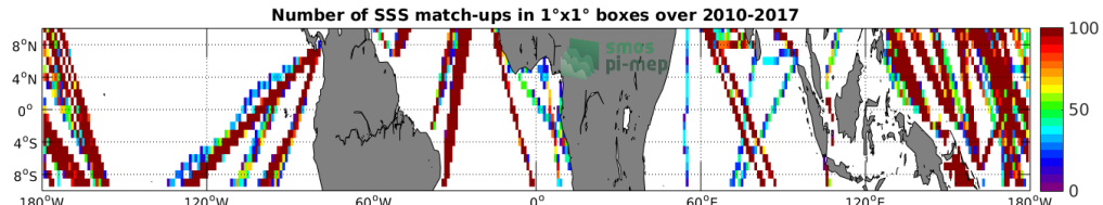
Figure 4: Number of SSS match-ups between TSG-LEGOS-DM SSS and the SMOS-L4-CATDS-CECOS-IFREMER-V2-WEEKLY-0.5DEG SSS product for the Equatorial Ocean 10N-10S Pi-MEP region over 1°x1° boxes and for the full satellite product period.
