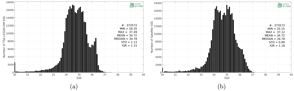
Figure 2: Histograms of SSS from TSG-LEGOS-DM (a) and SMOS-L4-CATDS-CECOS-IFREMER-V2-WEEKLY-0.5DEG (b) considering all match-up pairs per bins of 0.1 over the Equatorial Ocean 10N-10S Pi-MEP region and for the full satellite product period.
