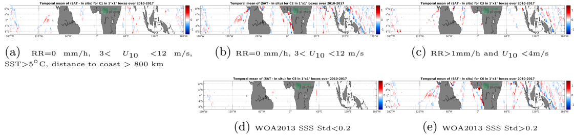
Figure 12: Temporal mean gridded over spatial boxes of size 1^\circ \times 1^\circ of \Delta SSS (SMOS-L4-CATDS-CECOS-IFREMER-V2-WEEKLY-0.5DEG - TSG-LEGOS-DM) for 5 different subdatasets corresponding to: RR=0 mm/h, 3 < U_{10} < 12 m/s, SST > 5^\circ C , distance to coast > 800 km (a), RR=0 mm/h, 3 < U_{10} < 12 m/s (b), RR > 1 mm/h and U_{10} < 4 m/s (c), WOA2013 SSS Std < 0.2 (d), WOA2013 SSS Std > 0.2 (e).
