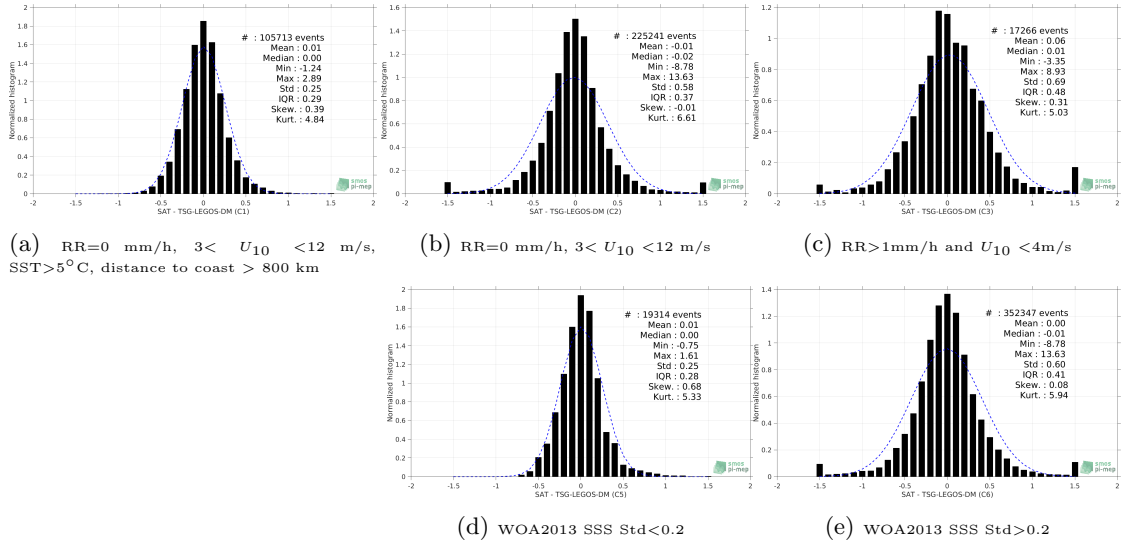
Figure 13: Normalized histogram of \Delta SSS (SMOS-L4-CATDS-CECOS-IFREMER-V2-WEEKLY-0.5DEG - TSG-LEGOS-DM) for 5 different subdatasets corresponding to: RR=0 mm/h, 3 < U_{10} < 12 m/s, SST > 5^\circ C , distance to coast > 800 km (a), RR=0 mm/h, 3 < U_{10} < 12 m/s (b), RR > 1 mm/h and U_{10} < 4 m/s (c), WOA2013 SSS Std < 0.2 (d), WOA2013 SSS Std > 0.2 (e).
