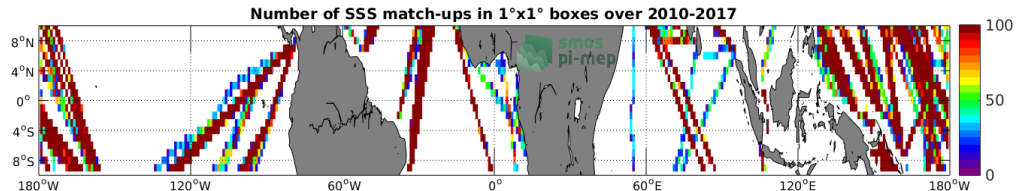
Figure 4: Number of SSS match-ups between TSG-LEGOS-DM SSS and the SMOS-L4-CATDS-CECOS-IFREMER-V2-WEEKLY-0.5DEG SSS product for the Equatorial Ocean 10N-10S Pi-MEP region over 1^\circ \times 1^\circ boxes and for the full satellite product period.
