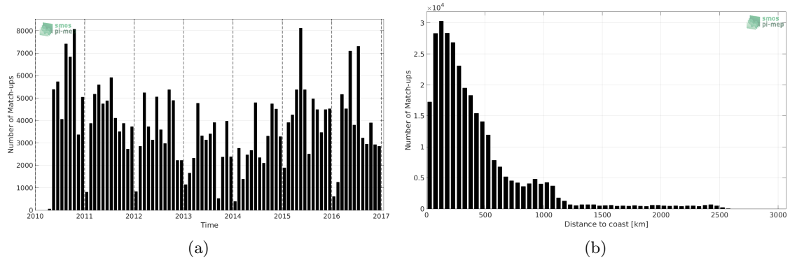
Figure 1: Number of match-ups between TSG-LEGOS-DM and SMOS-L4-CATDS-CECOS-IFREMER-V2-WEEKLY-0.5DEG SSS as a function of time (a) and as function of the distance to coast (b) over the Equatorial Ocean 10N-10S Pi-MEP region and for the full satellite product period.
