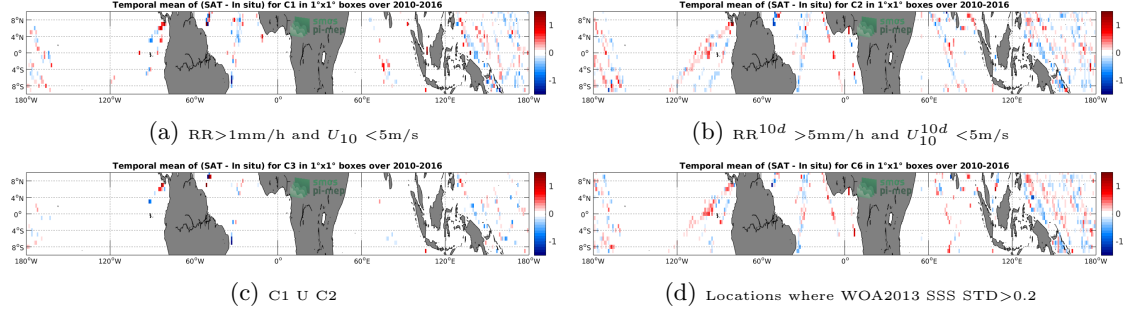
Figure 12: Temporal mean gridded over spatial boxes of size 1^\circ \times 1^\circ of \Delta SSS (SMOS-L4-CATDS-CECOS-IFREMER-V2-WEEKLY-0.5DEG - TSG-LEGOS-DM) for 4 different subdatasets corresponding to: RR > 1\text{mm/h} and U_{10} < 5\text{m/s} (a), RR^{10d} > 5\text{mm/h} and U_{10}^{10d} < 5\text{m/s} (b), C1 U C2 (c), Locations where WOA2013 SSS STD > 0.2 (d).
