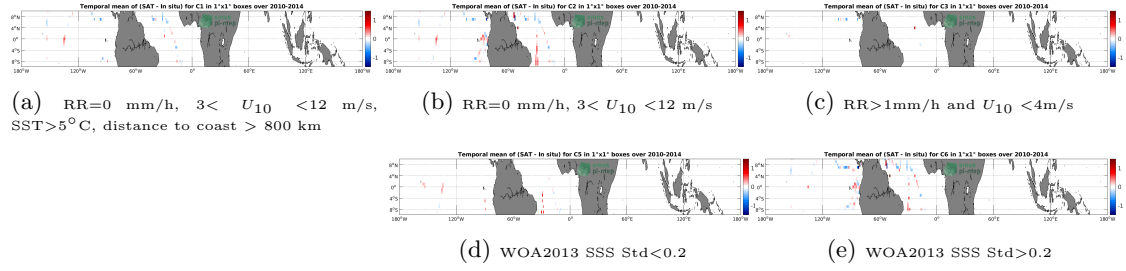
Figure 12: Temporal mean gridded over spatial boxes of size 1^{\circ}\times 1^{\circ} of \Delta SSS (SMOS L4 v2 Weekly (CATDS-CECOS-IFREMER) - TSG (GOSUD-Sailing-ship)) for 5 different subdatasets corresponding to: RR=0 mm/h, 3 < U_{10} < 12 m/s, SST > 5^{\circ}\text{C} , distance to coast > 800 km (a), RR=0 mm/h, 3 < U_{10} < 12 m/s (b), RR > 1 mm/h and U_{10} < 4 m/s (c), WOA2013 SSS Std < 0.2 (d), WOA2013 SSS Std > 0.2 (e).
