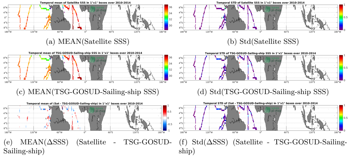
Figure 6: Temporal mean (left) and Std (right) of SSS from SMOS-L4-CATDS-CECOS-IFREMER-V2-WEEKLY-0.5DEG (top), TSG-GOSUD-Sailing-ship (middle), and of \Delta SSS (Satellite - TSG-GOSUD-Sailing-ship). Only match-up pairs are used to generate these maps.
