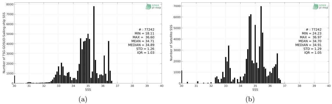
Figure 2: Histograms of SSS from TSG-GOSUD-Sailing-ship (a) and SMOS-L4-CATDS-CECOS-IFREMER-V2-WEEKLY-0.5DEG (b) considering all match-up pairs per bins of 0.1 over the Equatorial Ocean 10N-10S Pi-MEP region and for the full satellite product period.
