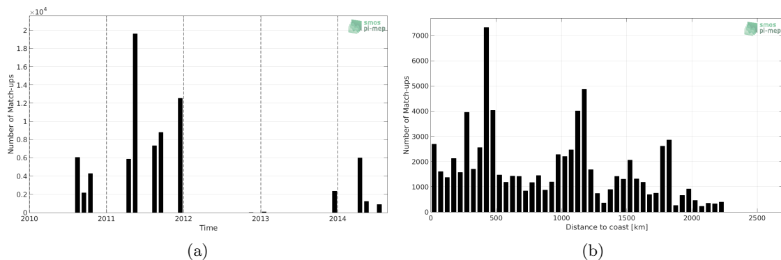
Figure 1: Number of match-ups between TSG-GOSUD-Sailing-ship and SMOS-L4-CATDS-CECOS-IFREMER-V2-WEEKLY-0.5DEG SSS as a function of time (a) and as function of the distance to coast (b) over the Equatorial Ocean 10N-10S Pi-MEP region and for the full satellite product period.
