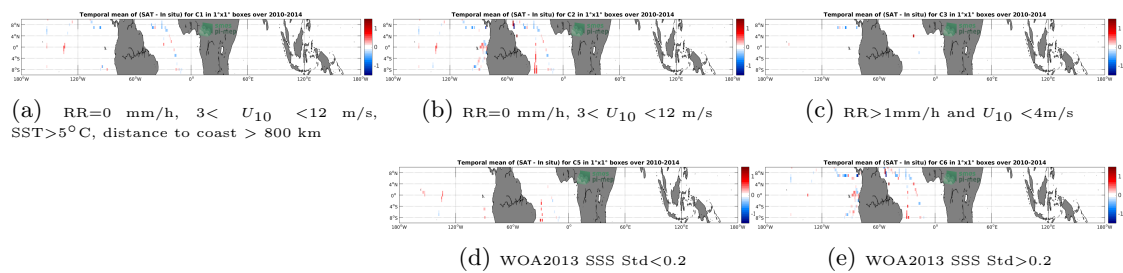
Figure 12: Temporal mean gridded over spatial boxes of size 1^\circ \times 1^\circ of \Delta SSS (SMOS-L4-CATDS-CECOS-IFREMER-V2-WEEKLY-0.5DEG - TSG-GOSUD-Sailing-ship) for 5 different subdatasets corresponding to: RR=0 mm/h, 3 < U_{10} < 12 m/s, SST > 5^\circ\text{C} , distance to coast > 800 km (a), RR=0 mm/h, 3 < U_{10} < 12 m/s (b), RR > 1 mm/h and U_{10} < 4 m/s (c), WOA2013 SSS Std < 0.2 (d), WOA2013 SSS Std > 0.2 (e).
