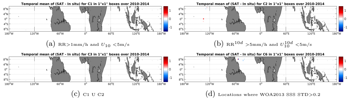
Figure 12: Temporal mean gridded over spatial boxes of size 1^\circ \times 1^\circ of \Delta SSS (SMOS-L4-CATDS-CECOS-IFREMER-V2-WEEKLY-0.5DEG - TSG-GOSUD-Sailing-ship) for 4 different subdatasets corresponding to: RR > 1\text{mm/h} and U_{10} < 5\text{m/s} (a), RR^{10d} > 5\text{mm/h} and U_{10}^{10d} < 5\text{m/s} (b), C1 U C2 (c), Locations where WOA2013 SSS STD > 0.2 (d).
