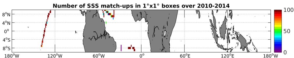
Figure 4: Number of SSS match-ups between TSG-GOSUD-Sailing-ship SSS and the SMOS-L4-CATDS-CECOS-IFREMER-V2-WEEKLY-0.5DEG SSS product for the Equatorial Ocean 10N-10S Pi-MEP region over 1^{\circ} \times 1^{\circ} boxes and for the full satellite product period.
