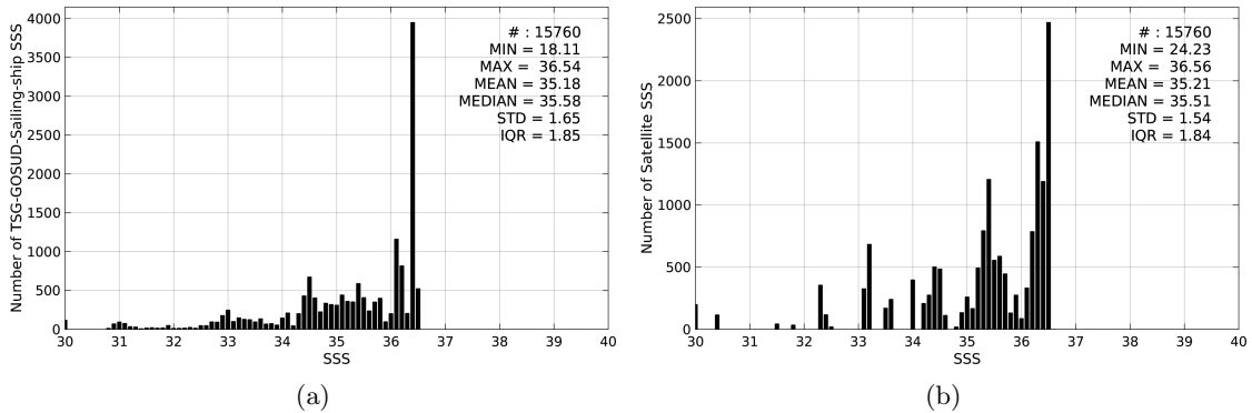
Figure 2: Histograms of SSS from TSG-GOSUD-Sailing-ship (a) and SMOS-L4-CATDS-CECOS-IFREMER-V2-WEEKLY-0.5DEG (b) considering all match-up pairs per bins of 0.1 over the Equatorial Ocean 10N-10S Pi-MEP region and for the full satellite product period.
