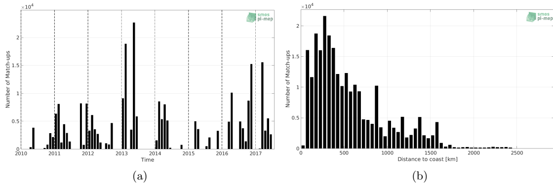
Figure 1: Number of match-ups between TSG (GOSUD-Research-vessel) and SMOS L4 v2 Weekly (CATDS-CECOS-IFREMER) SSS as a function of time (a) and as function of the distance to coast (b) over the Equatorial Ocean 10N-10S Pi-MEP region and for the full satellite product period.
