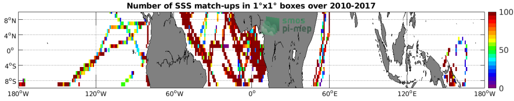
Figure 4: Number of SSS match-ups between TSG (GOSUD-Research-vessel) SSS and the SMOS L4 v2 Weekly (CATDS-CECOS-IFREMER) SSS product for the Equatorial Ocean 10N-10S Pi-MEP region over 1^\circ \times 1^\circ boxes and for the full satellite product period.
