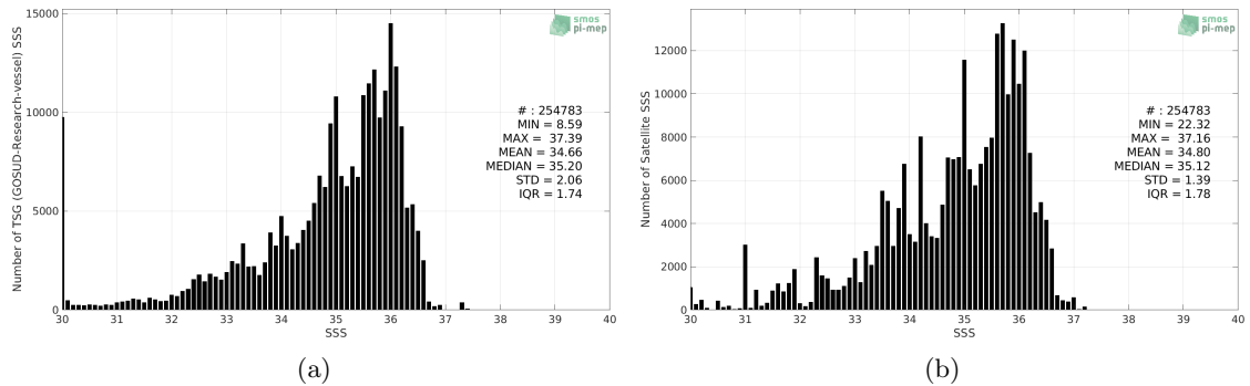
Figure 2: Histograms of SSS from TSG (GOSUD-Research-vessel) (a) and SMOS L4 v2 Weekly (CATDS-CECOS-IFREMER) (b) considering all match-up pairs per bins of 0.1 over the Equatorial Ocean 10N-10S Pi-MEP region and for the full satellite product period.
