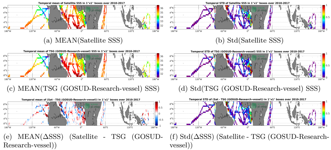
Figure 6: Temporal mean (left) and Std (right) of SSS from SMOS L4 v2 Weekly (CATDS-CECOS-IFREMER) (top), TSG (GOSUD-Research-vessel) (middle), and of \Delta SSS (Satellite - TSG (GOSUD-Research-vessel)). Only match-up pairs are used to generate these maps.
