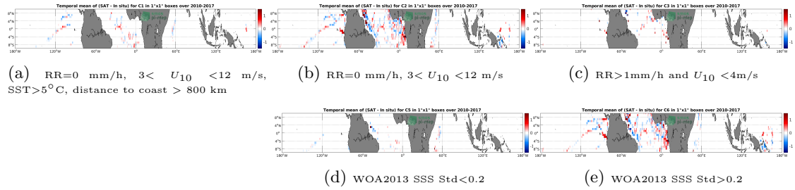
Figure 12: Temporal mean gridded over spatial boxes of size 1^{\circ}\times 1^{\circ} of \Delta SSS (SMOS L4 v2 Weekly (CATDS-CECOS-IFREMER) - TSG (GOSUD-Research-vessel)) for 5 different subdatasets corresponding to: RR=0 mm/h, 3 < U_{10} < 12 m/s, SST >5^{\circ}\text{C} , distance to coast > 800 km (a), RR=0 mm/h, 3 < U_{10} < 12 m/s (b), RR >1 mm/h and U_{10} < 4 m/s (c), WOA2013 SSS Std <0.2 (d), WOA2013 SSS Std >0.2 (e).
