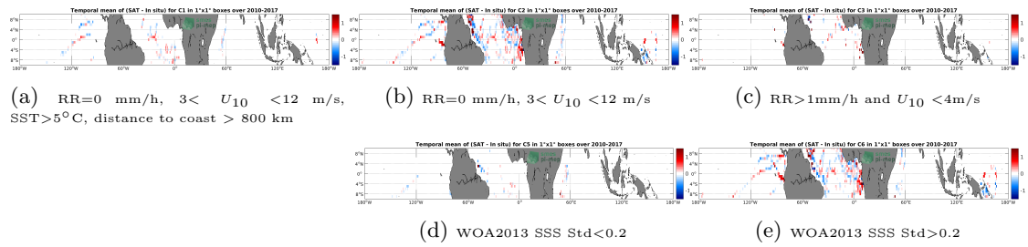
Figure 12: Temporal mean gridded over spatial boxes of size 1^{\circ}\times 1^{\circ} of \Delta SSS (SMOS L4 v2 Weekly (CATDS-CECOS-IFREMER) - TSG (GOSUD-Research-vessel)) for 5 different subdatasets corresponding to: RR=0 mm/h, 3 < U_{10} < 12 m/s, SST > 5^{\circ}\text{C} , distance to coast > 800 km (a), RR=0 mm/h, 3 < U_{10} < 12 m/s (b), RR > 1 mm/h and U_{10} < 4 m/s (c), WOA2013 SSS Std < 0.2 (d), WOA2013 SSS Std > 0.2 (e).
