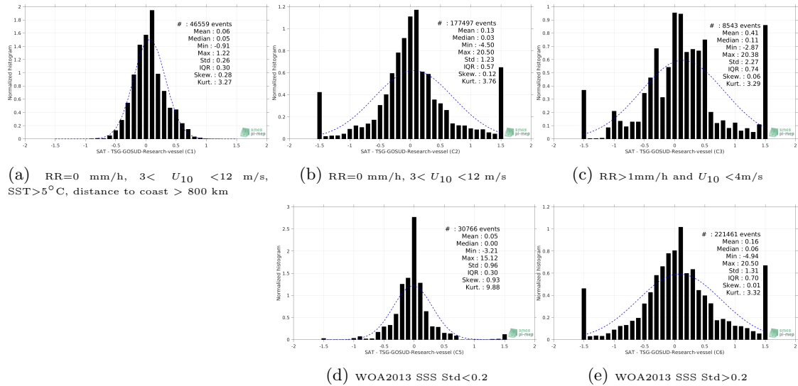
Figure 13: Normalized histogram of \Delta SSS (SMOS-L4-CATDS-CECOS-IFREMER-V2-WEEKLY-0.5DEG - TSG-GOSUD-Research-vessel) for 5 different sub-datasets corresponding to: RR=0 mm/h, 3 < U_{10} < 12 m/s, SST >5^\circ\text{C} , distance to coast > 800 km (a), RR=0 mm/h, 3 < U_{10} < 12 m/s (b), RR >1 mm/h and U_{10} < 4 m/s (c), WOA2013 SSS Std <0.2 (d), WOA2013 SSS Std >0.2 (e).
