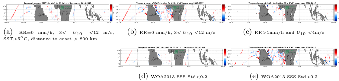
Figure 12: Temporal mean gridded over spatial boxes of size 1^\circ \times 1^\circ of \Delta SSS (SMOS-L4-CATDS-CECOS-IFREMER-V2-WEEKLY-0.5DEG - TSG-GOSUD-Research-vessel) for 5 different sub-datasets corresponding to: RR=0 mm/h, 3 < U_{10} < 12 m/s, SST >5^\circ\text{C} , distance to coast > 800 km (a), RR=0 mm/h, 3 < U_{10} < 12 m/s (b), RR >1 mm/h and U_{10} < 4 m/s (c), WOA2013 SSS Std <0.2 (d), WOA2013 SSS Std >0.2 (e).
