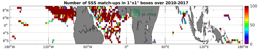
Figure 3: Number of SSS match-ups between Surface drifters SSS and the SMOS L4 v2 Weekly (CATDS-CECOS-IFREMER) SSS product for the Equatorial Ocean 10N-10S Pi-MEP region over 1^\circ \times 1^\circ boxes and for the full satellite product period.
