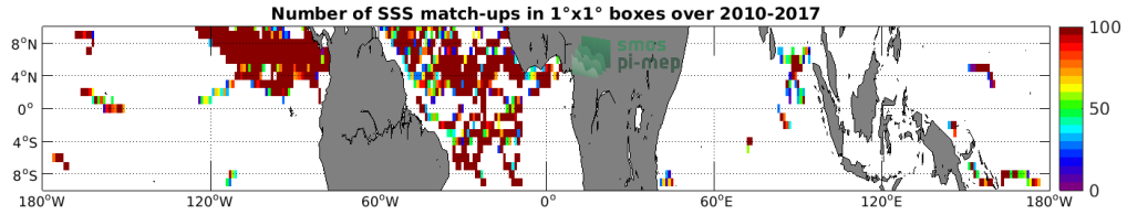
Figure 3: Number of SSS match-ups between Surface drifters SSS and the SMOS L4 v2 Weekly (CATDS-CECOS-IFREMER) SSS product for the Equatorial Ocean 10N-10S Pi-MEP region over 1°x1° boxes and for the full satellite product period.
