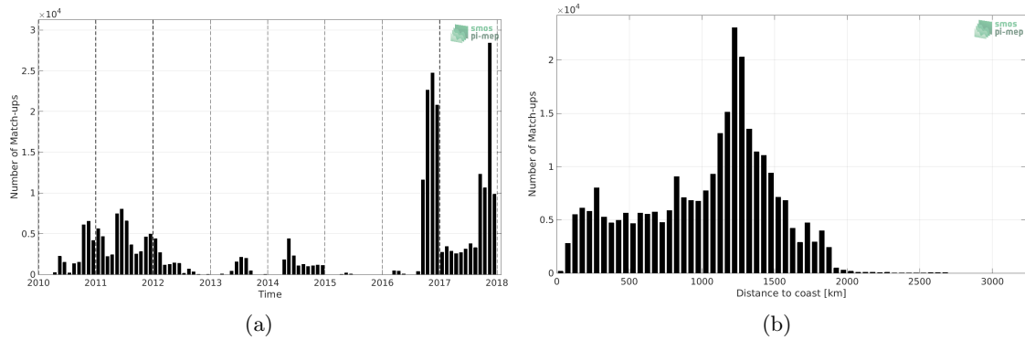
Figure 1: Number of match-ups between Surface drifters and SMOS L4 v2 Weekly (CATDS-CECOS-IFREMER) SSS as a function of time (a) and as function of the distance to coast (b) over the Equatorial Ocean 10N-10S Pi-MEP region and for the full satellite product period.
