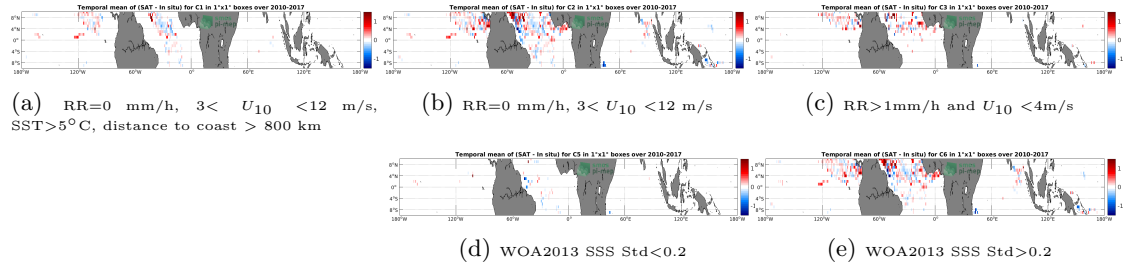
Figure 11: Temporal mean gridded over spatial boxes of size 1^{\circ}\times 1^{\circ} of \Delta\text{SSS} (SMOS L4 v2 Weekly (CATDS-CECOS-IFREMER) - Surface drifters) for 5 different subdatasets corresponding to:RR=0 mm/h, 3 < U_{10} < 12 m/s, SST >5^{\circ}\text{C} , distance to coast > 800 km (a), RR=0 mm/h, 3 < U_{10} < 12 m/s (b), RR >1 mm/h and U_{10} < 4 m/s (c), WOA2013 SSS Std <0.2 (d), WOA2013 SSS Std >0.2 (e).
