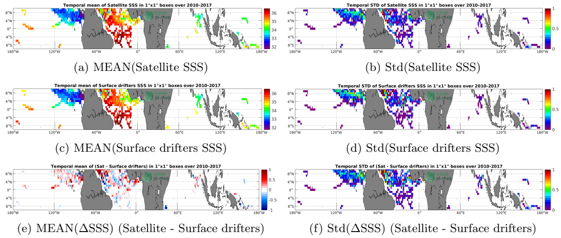
Figure 5: Temporal mean (left) and Std (right) of SSS from SMOS L4 v2 Weekly (CATDS-CECOS-IFREMER) (top), Surface drifters (middle), and of \Delta SSS (Satellite - Surface drifters). Only match-up pairs are used to generate these maps.
