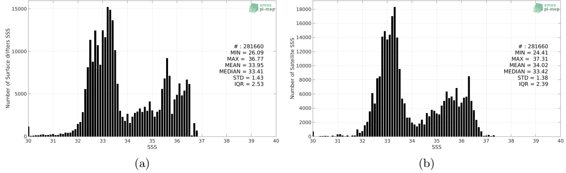
Figure 2: Histograms of SSS from Surface drifters (a) and SMOS L4 v2 Weekly (CATDS-CECOS-IFREMER) (b) considering all match-up pairs per bins of 0.1 over the Equatorial Ocean 10N-10S Pi-MEP region and for the full satellite product period.
