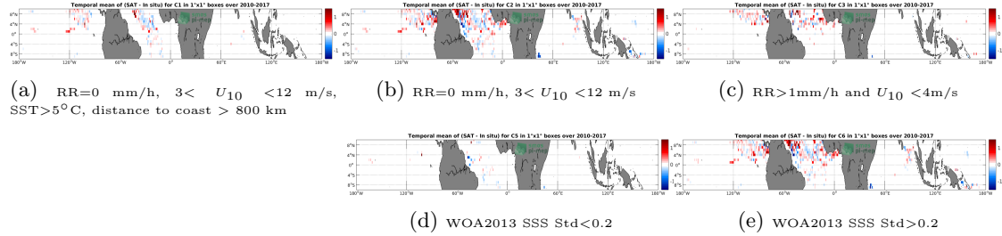
Figure 11: Temporal mean gridded over spatial boxes of size 1^{\circ}\times 1^{\circ} of \Delta\text{SSS} (SMOS-L4-CATDS-CECOS-IFREMER-V2-WEEKLY-0.5DEG - Surface drifters) for 5 different subdatasets corresponding to:RR=0 mm/h, 3 < U_{10} < 12 m/s, SST >5^{\circ}\text{C} , distance to coast > 800 km (a), RR=0 mm/h, 3 < U_{10} < 12 m/s (b), RR >1 mm/h and U_{10} < 4 m/s (c), WOA2013 SSS Std <0.2 (d), WOA2013 SSS Std >0.2 (e).
