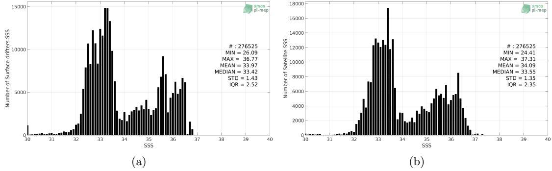
Figure 2: Histograms of SSS from Surface drifters (a) and SMOS-L4-CATDS-CECOS-IFREMER-V2-WEEKLY-0.5DEG (b) considering all match-up pairs per bins of 0.1 over the Equatorial Ocean 10N-10S Pi-MEP region and for the full satellite product period.
