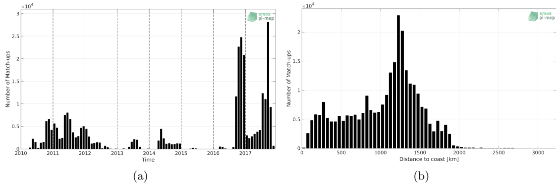
Figure 1: Number of match-ups between Surface drifters and SMOS-L4-CATDS-CECOS-IFREMER-V2-WEEKLY-0.5DEG SSS as a function of time (a) and as function of the distance to coast (b) over the Equatorial Ocean 10N-10S Pi-MEP region and for the full satellite product period.
