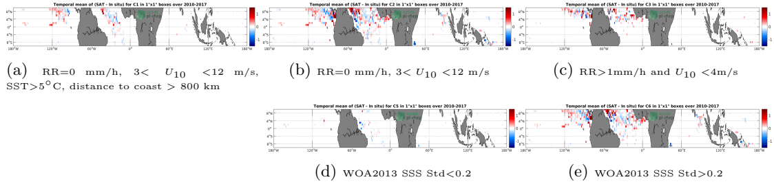
Figure 11: Temporal mean gridded over spatial boxes of size 1^\circ \times 1^\circ of \Delta SSS (SMOS-L4-CATDS-CECOS-IFREMER-V2-WEEKLY-0.5DEG - Surface drifters) for 5 different subdatasets corresponding to:RR=0 mm/h, 3 < U_{10} < 12 m/s, SST >5^\circ C, distance to coast > 800 km (a), RR=0 mm/h, 3 < U_{10} < 12 m/s (b), RR >1 mm/h and U_{10} < 4 m/s (c), WOA2013 SSS Std <0.2 (d), WOA2013 SSS Std >0.2 (e).
