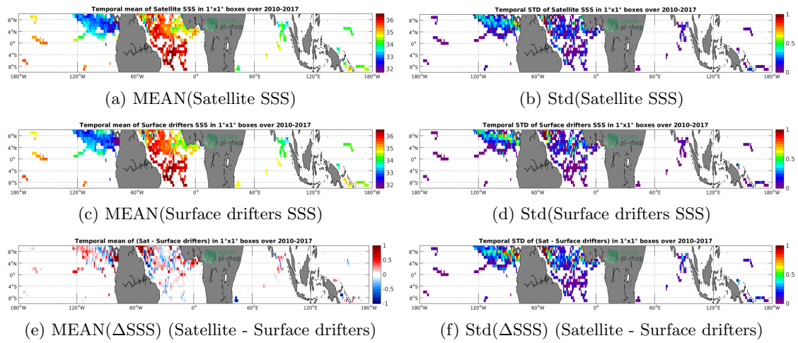
Figure 5: Temporal mean (left) and Std (right) of SSS from SMOS-L4-CATDS-CECOS-IFREMER-V2-WEEKLY-0.5DEG (top), Surface drifters (middle), and of \Delta SSS (Satellite - Surface drifters). Only match-up pairs are used to generate these maps.
