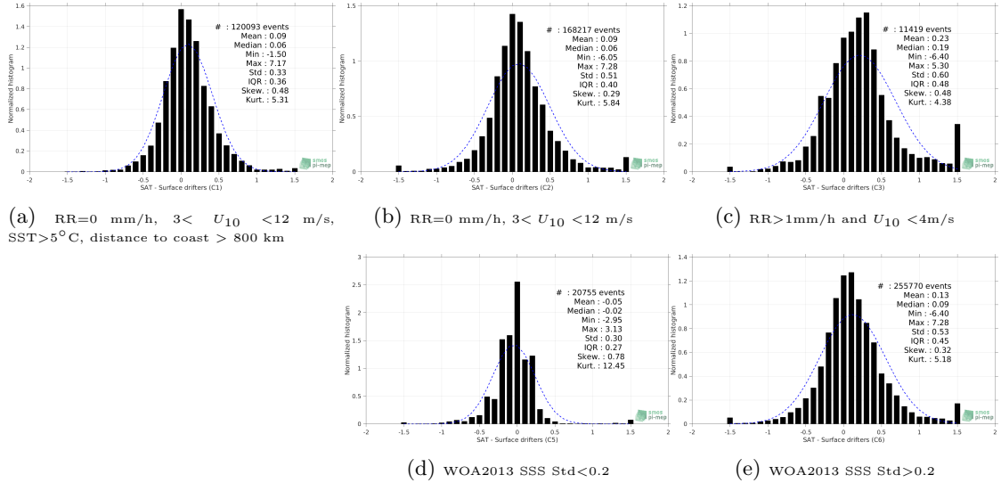
Figure 12: Normalized histogram of \Delta SSS (SMOS-L4-CATDS-CECOS-IFREMER-V2-WEEKLY-0.5DEG - Surface drifters) for 5 different subdatasets corresponding to: RR=0 mm/h, 3 < U_{10} < 12 m/s, SST >5^\circ C, distance to coast > 800 km (a), RR=0 mm/h, 3 < U_{10} < 12 m/s (b), RR >1 mm/h and U_{10} < 4 m/s (c), WOA2013 SSS Std <0.2 (d), WOA2013 SSS Std >0.2 (e).
