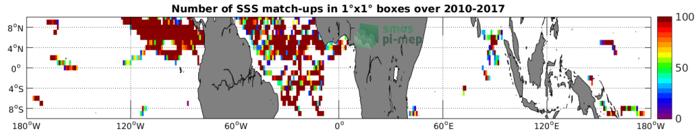
Figure 3: Number of SSS match-ups between Surface drifters SSS and the SMOS-L4-CATDS-CECOS-IFREMER-V2-WEEKLY-0.5DEG SSS product for the Equatorial Ocean 10N-10S Pi-MEP region over 1^\circ \times 1^\circ boxes and for the full satellite product period.
