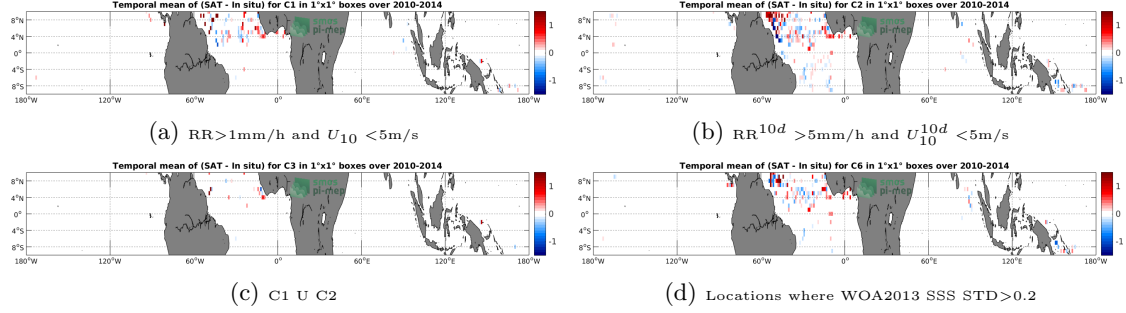
Figure 11: Temporal mean gridded over spatial boxes of size 1^\circ \times 1^\circ of \Delta SSS (SMOS-L4-CATDS-CECOS-IFREMER-V2-WEEKLY-0.5DEG - Surface drifters) for 4 different subdatasets corresponding to: RR > 1\text{mm/h} and U_{10} < 5\text{m/s} (a), RR^{10d} > 5\text{mm/h} and U_{10}^{10d} < 5\text{m/s} (b), C1 U C2 (c), Locations where WOA2013 SSS STD > 0.2 (d).
