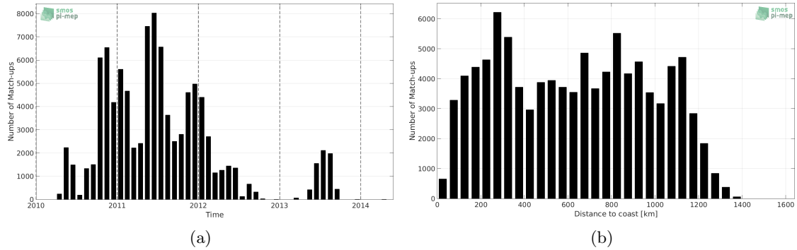
Figure 1: Number of match-ups between Surface drifters and SMOS-L4-CATDS-CECOS-IFREMER-V2-WEEKLY-0.5DEG SSS as a function of time (a) and as function of the distance to coast (b) over the Equatorial Ocean 10N-10S Pi-MEP region and for the full satellite product period.
