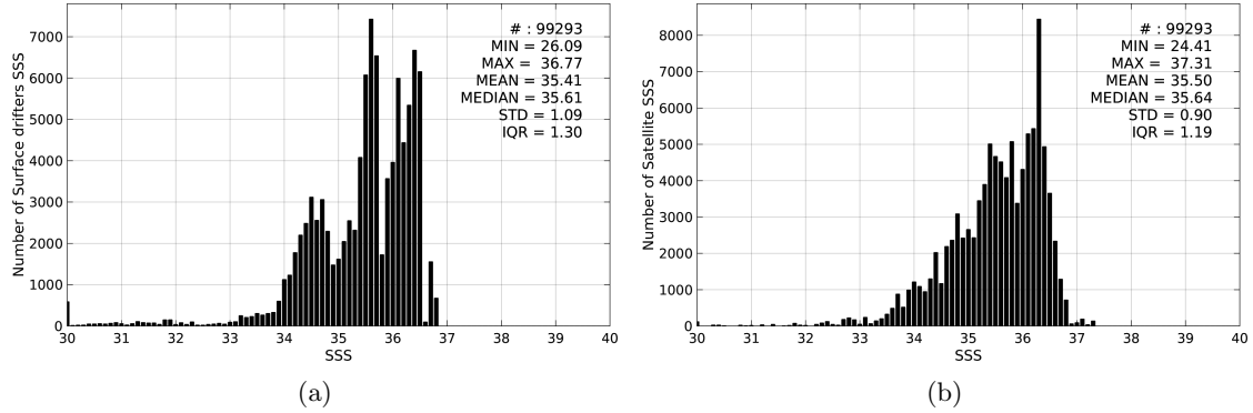
Figure 2: Histograms of SSS from Surface drifters (a) and SMOS-L4-CATDS-CECOS-IFREMER-V2-WEEKLY-0.5DEG (b) considering all match-up pairs per bins of 0.1 over the Equatorial Ocean 10N-10S Pi-MEP region and for the full satellite product period.
