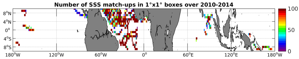
Figure 3: Number of SSS match-ups between Surface drifters SSS and the SMOS-L4-CATDS-CECOS-IFREMER-V2-WEEKLY-0.5DEG SSS product for the Equatorial Ocean 10N-10S Pi-MEP region over 1°x1° boxes and for the full satellite product period.
