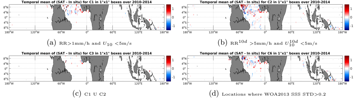
Figure 11: Temporal mean gridded over spatial boxes of size 1^\circ \times 1^\circ of \Delta SSS (SMOS-L4-CATDS-CECOS-IFREMER-V2-WEEKLY-0.5DEG - Surface drifters) for 4 different subdatasets corresponding to: RR > 1 mm/h and U_{10} < 5 m/s (a), RR^{10d} > 5 mm/h and U_{10}^{10d} < 5 m/s (b), C1 U C2 (c), Locations where WOA2013 SSS STD > 0.2 (d).
