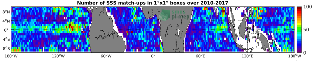
Figure 4: Number of SSS match-ups between Argo SSS and the SMOS L4 v2 Weekly (CATDS-CECOS-IFREMER) SSS product for the Equatorial Ocean 10N-10S Pi-MEP region over 1^\circ \times 1^\circ boxes and for the full satellite product period.
